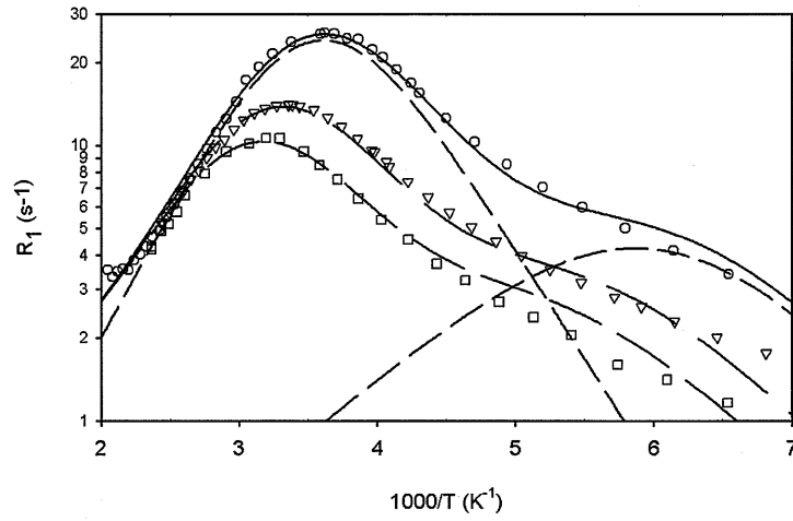
Figure 2. Fit of the relaxation data for x=4.0 . Symbols are experimental data: circles 37.3 MHz, triangles 67.7 MHz, squares 90.0 MHz. The continuous lines are the fit to the data (including the electronic relaxation contribution). The dashed lines are the ee contribution (left hand peak) and the eg contribution (right hand peak) to the relaxation rate given by equn. (30) for the 37.3 MHz data.
