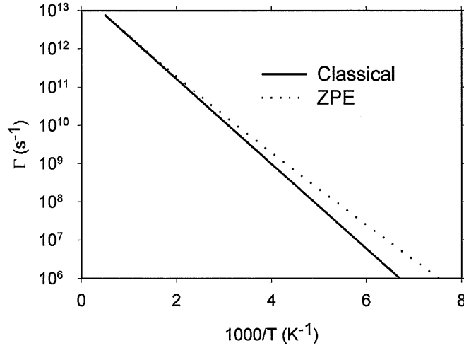
Figure 1. The hopping rate \Gamma as a function of 1000/T for e to g hops. The classical result is from equn.(22), the inclusion of zero point energy effects is from equn.(23).
