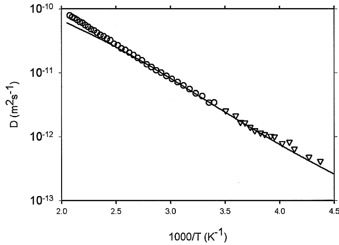
Figure 3. Fit to the diffusivity data for x=4.0 for the same parameters as in Fig. 2. The symbols are the experimental data. The solid line is the calculated D using equns. (20) and (21).
