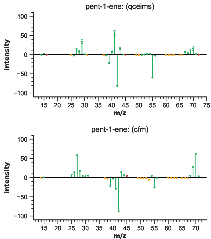
Figure S24: EIMS differences for pent-1-ene
