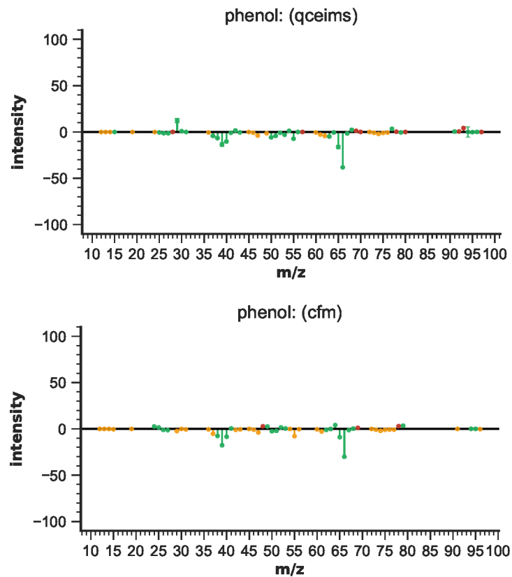
Figure S108: EIMS differences for phenol
