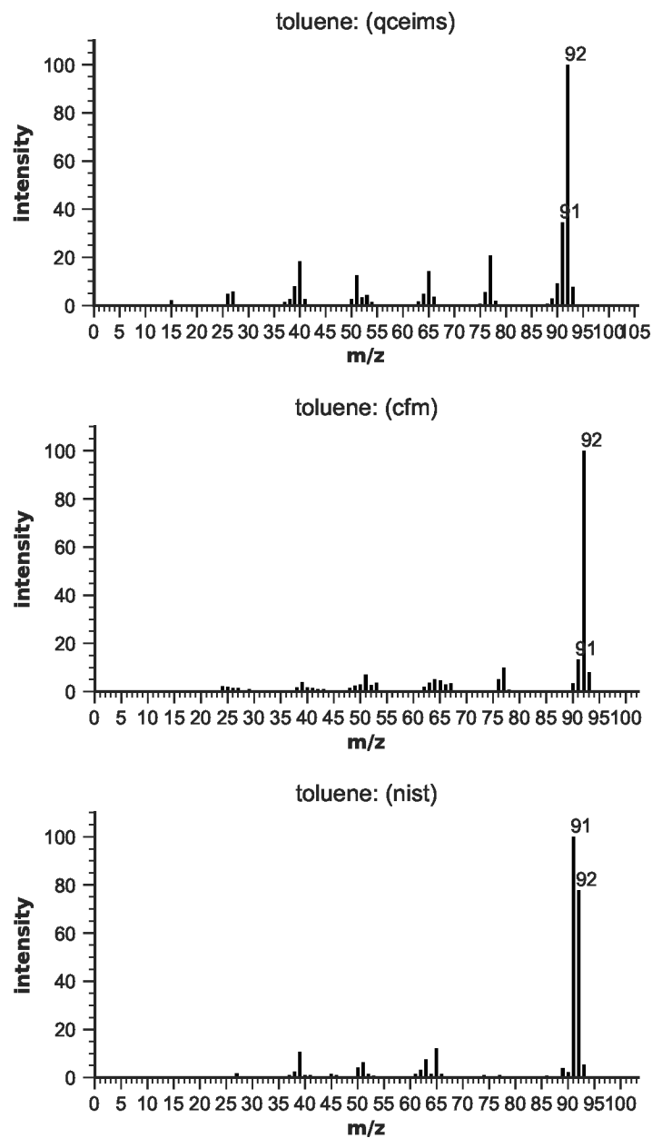
Figure S47: EIMS for toluene
