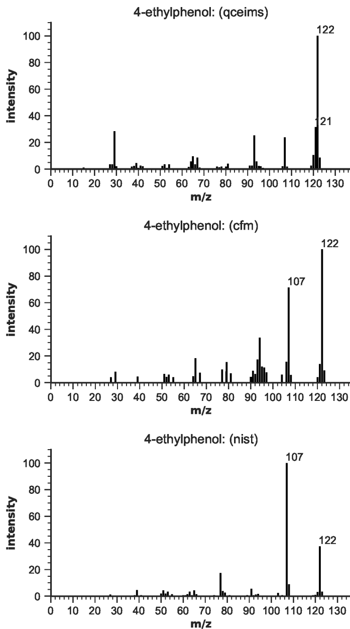
Figure S111: EIMS for 4-ethylphenol
