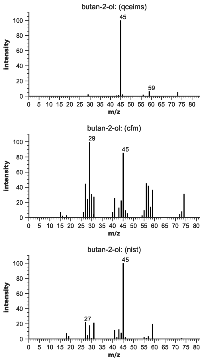
Figure S7: EIMS for butan-2-ol
