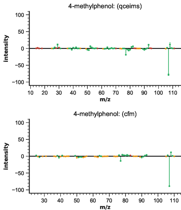
Figure S110: EIMS differences for 4-methylphenol
