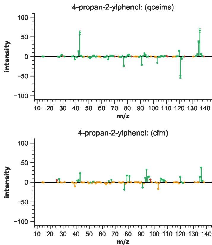
Figure S116: EIMS differences for 4-propan-2-ylphenol
