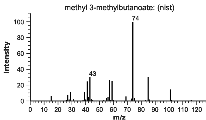
Figure S97: EIMS for methyl 3-methylbutanoate
