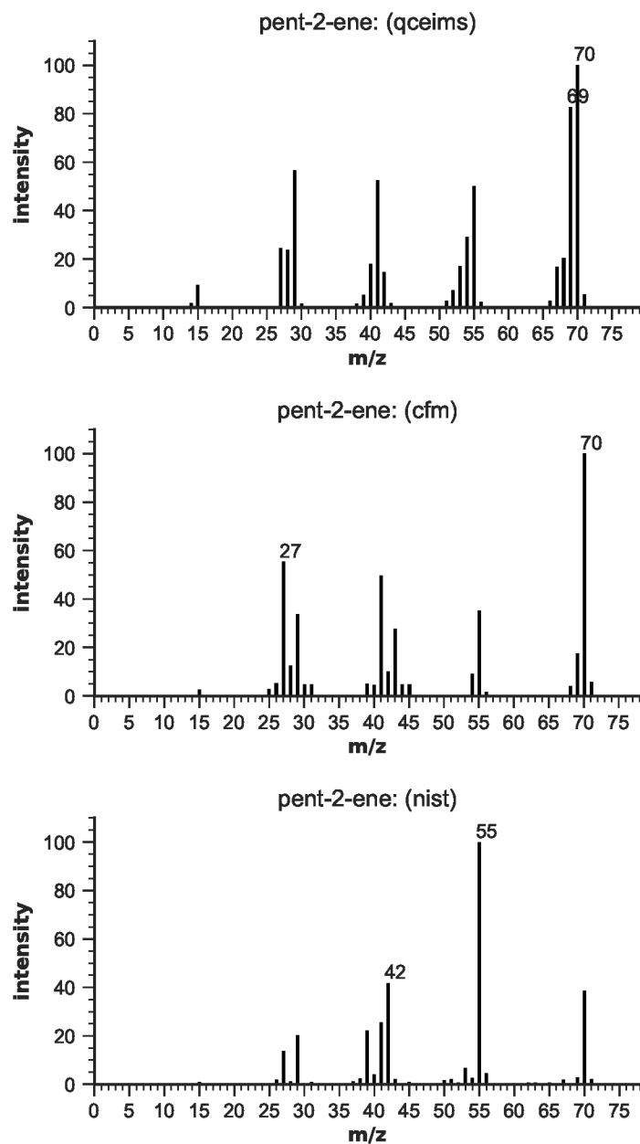
Figure S25: EIMS for pent-2-ene
