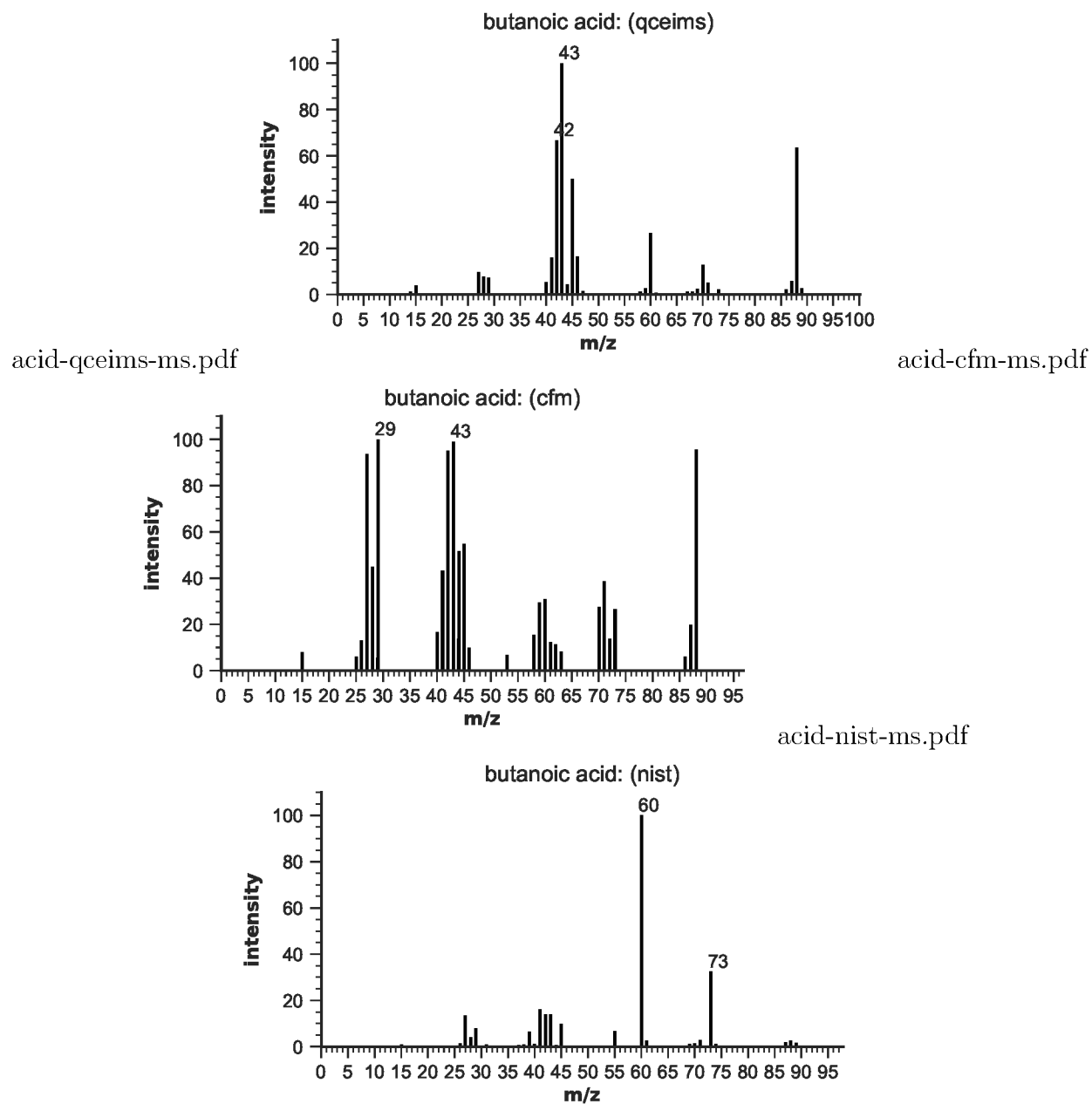
Figure S63: EIMS for butanoic acid
