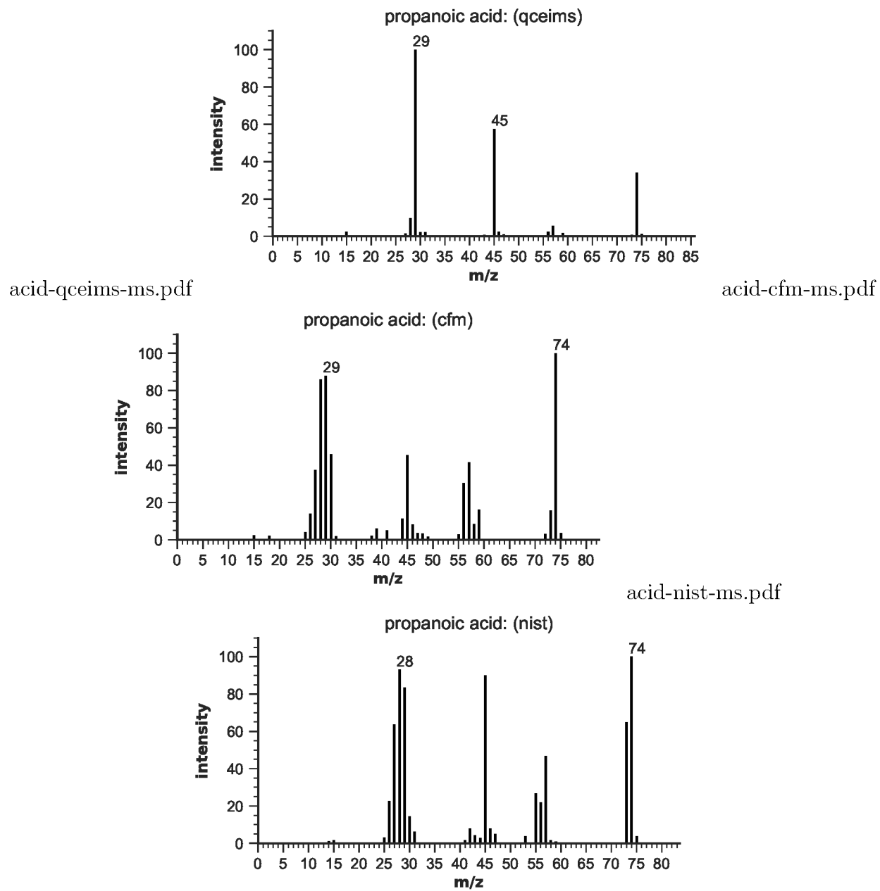
Figure S61: EIMS for propanoic acid
