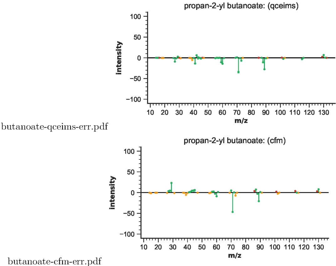
Figure S102: EIMS differences for propan-2-yl butanoate
