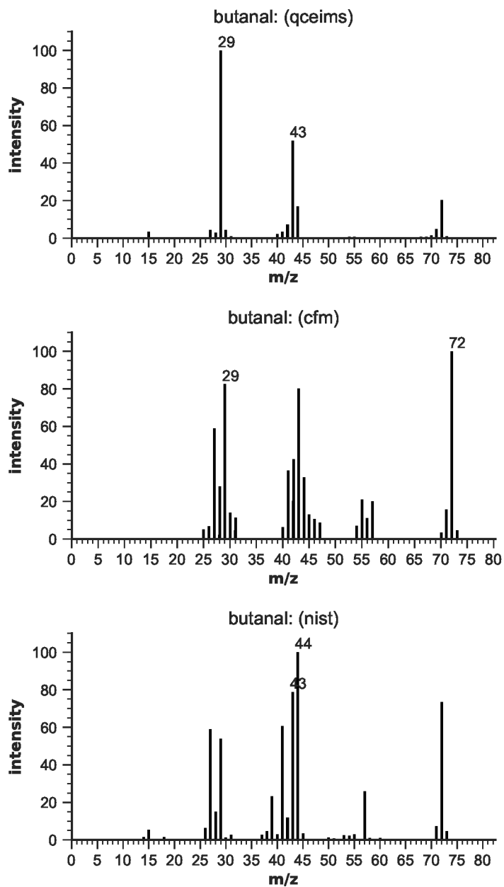
Figure S17: EIMS for butanal
