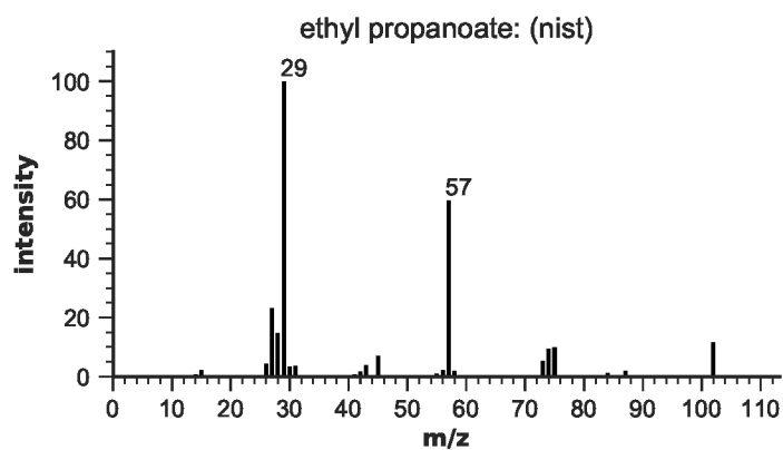
Figure S85: EIMS for ethyl propanoate
