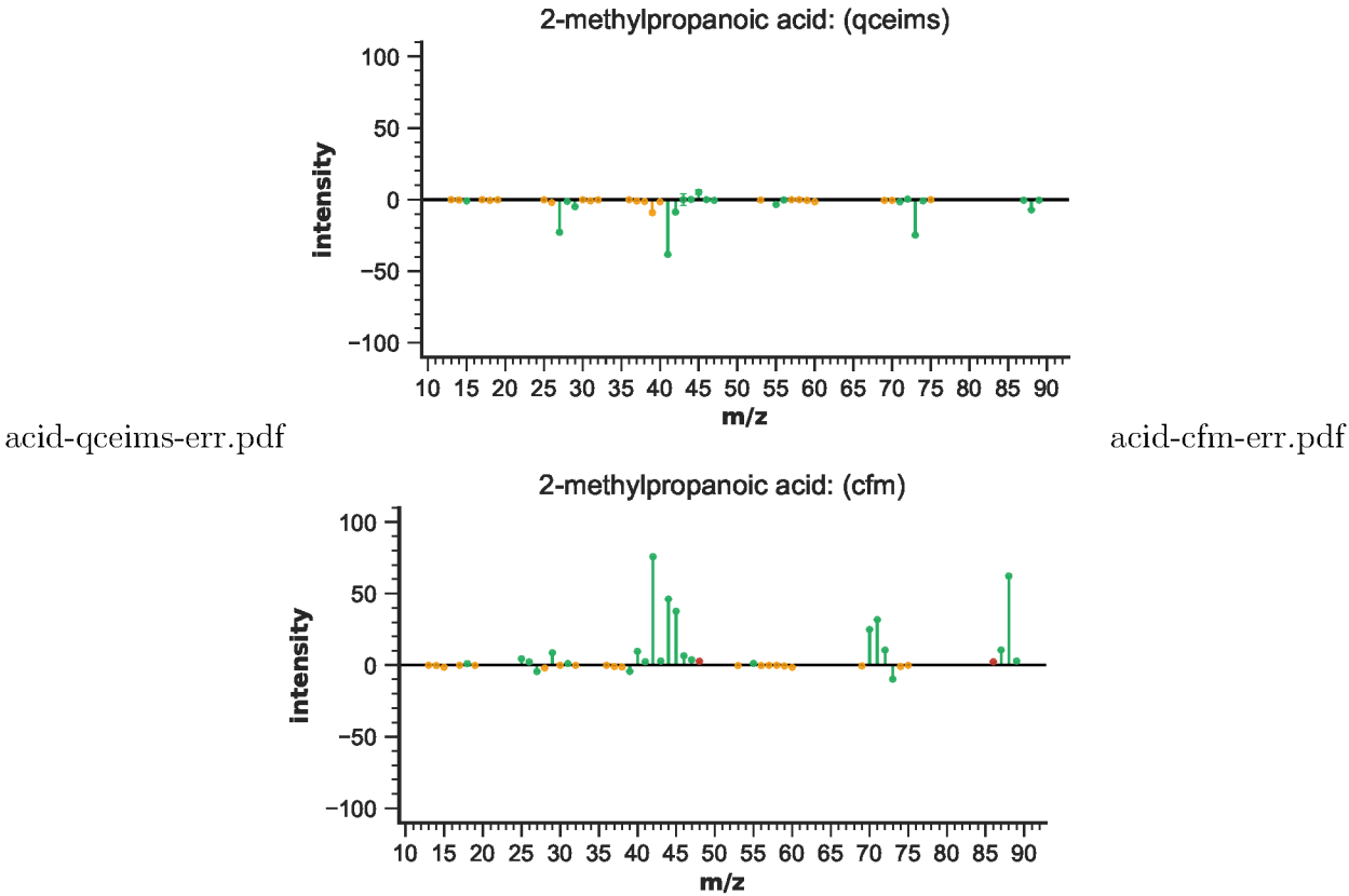
Figure S66: EIMS differences for 2-methylpropanoic acid
