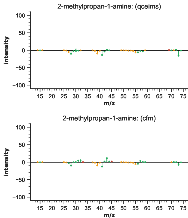
Figure S42: EIMS differences for 2-methylpropan-1-amine
