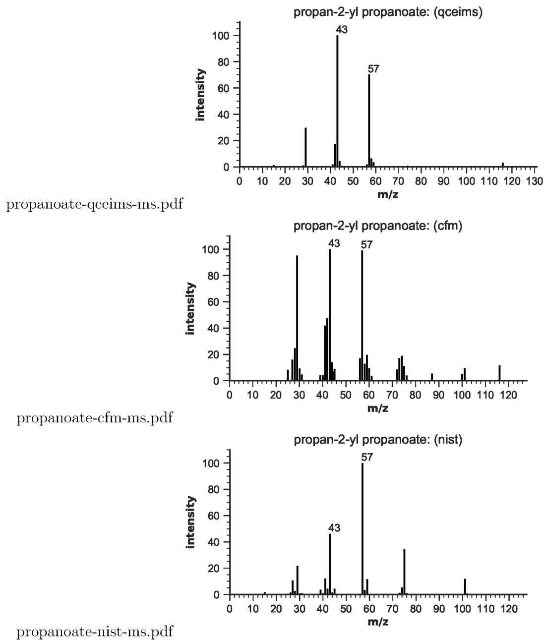
Figure S91: EIMS for propan-2-yl propanoate
