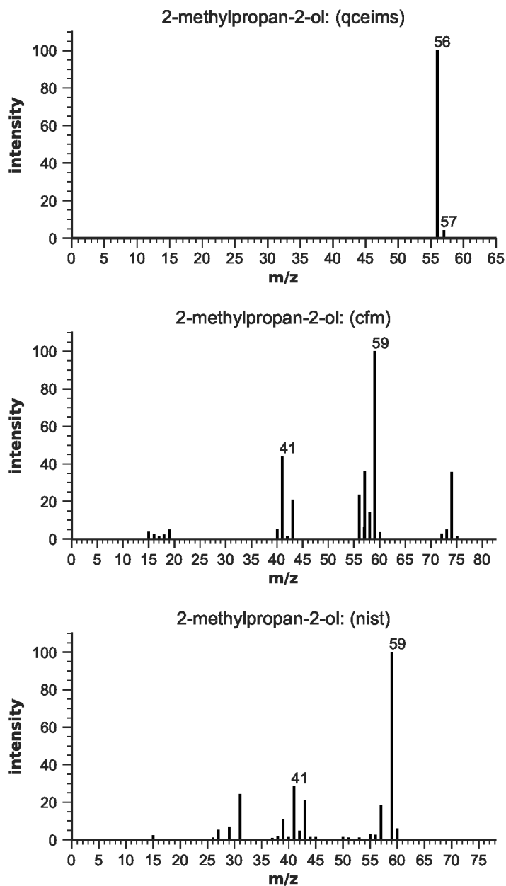
Figure S11: EIMS for 2-methylpropan-2-ol
