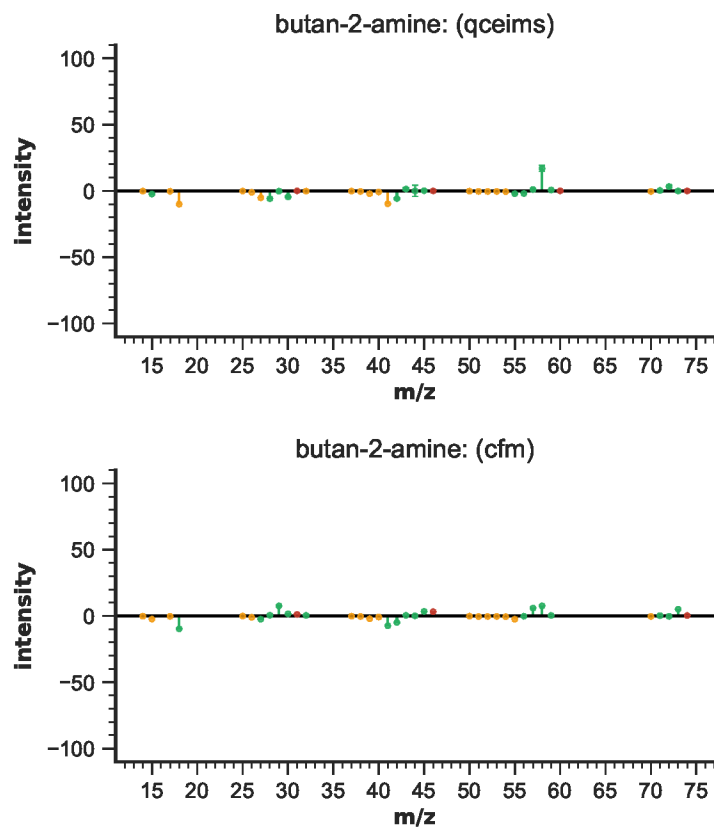
Figure S40: EIMS differences for butan-2-amine
