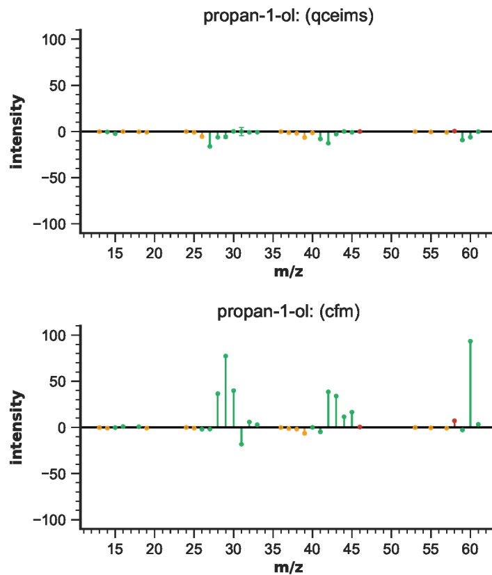
Figure S2: EIMS differences for propan-1-ol
