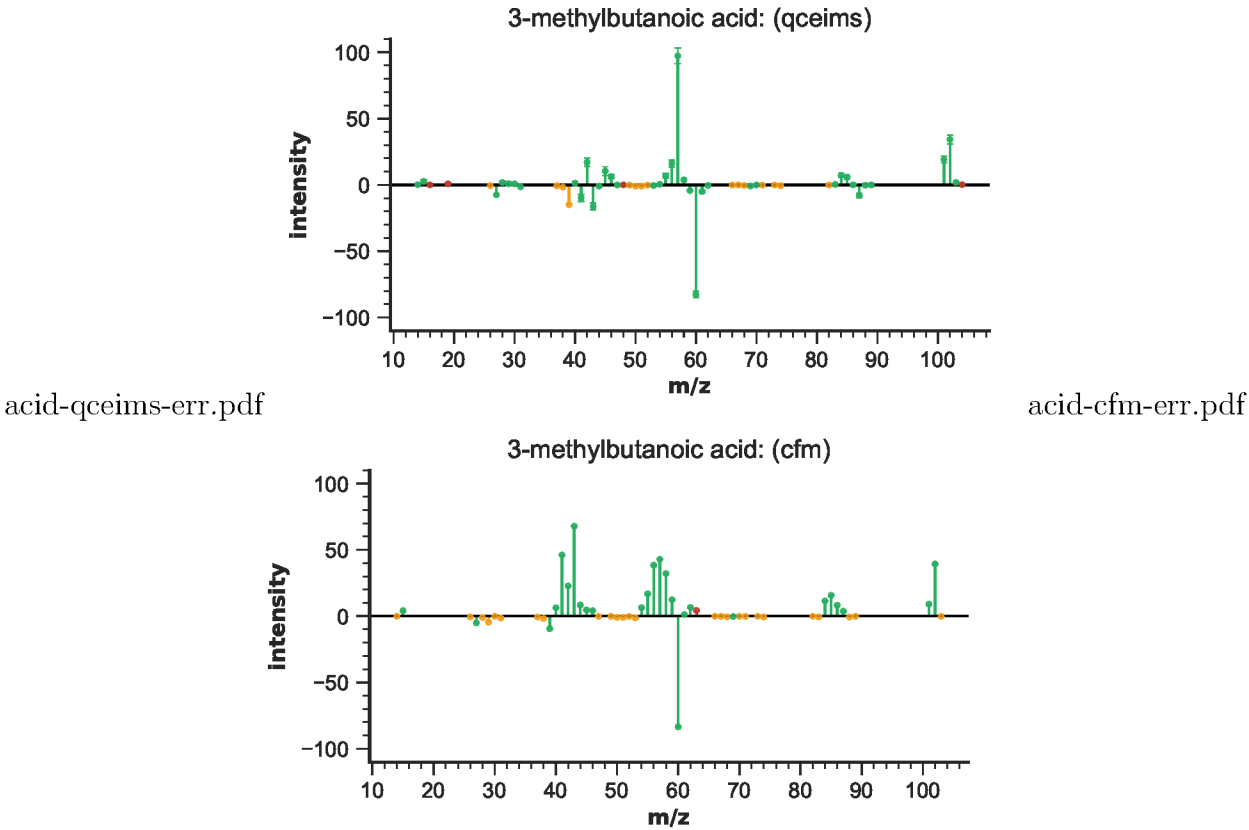
Figure S70: EIMS differences for 3-methylbutanoic acid
