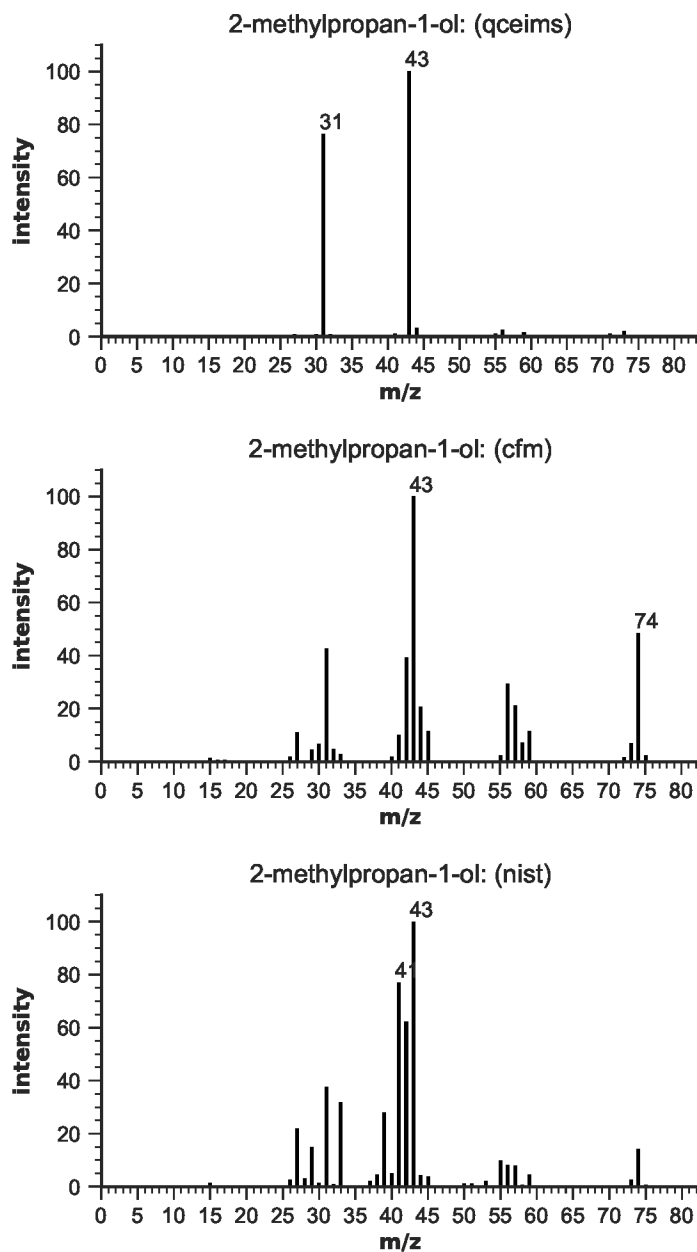
Figure S9: EIMS for 2-methylpropan-1-ol
