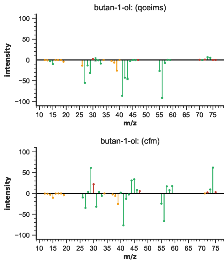
Figure S6: EIMS differences for butan-1-ol
