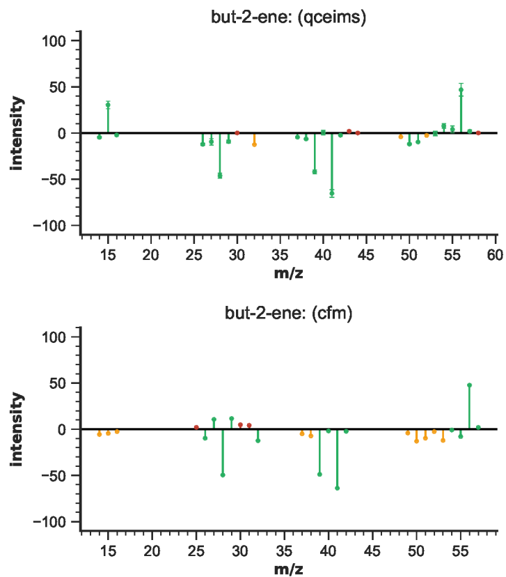
Figure S22: EIMS differences for but-2-ene
