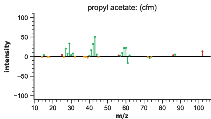
Figure S80: EIMS differences for propyl acetate
