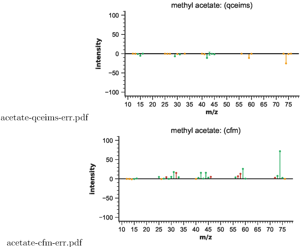
Figure S74: EIMS differences for methyl acetate
