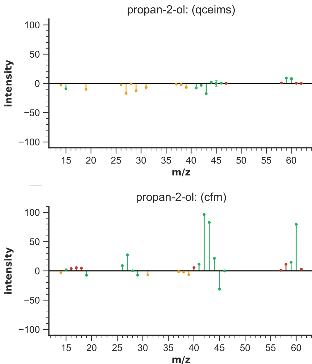
Figure 3: Difference between predicted (QCEIMS/CFM-EI) and experimental (NIST) spectra. Green bars indicate the presence of a correct peak, yellow indicates a missing peak, and red indicates a peak which is incorrect i.e. should not have been predicted.
