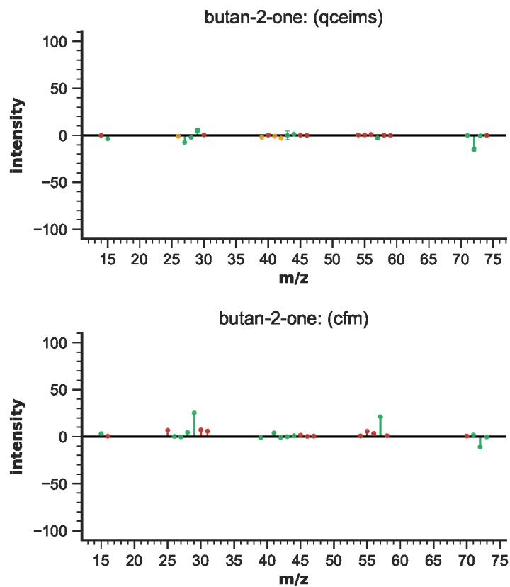
Figure S106: EIMS differences for butan-2-one
