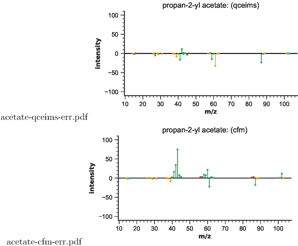
Figure S82: EIMS differences for propan-2-yl acetate
