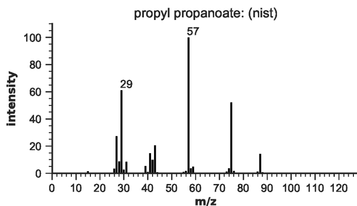
Figure S89: EIMS for propyl propanoate
