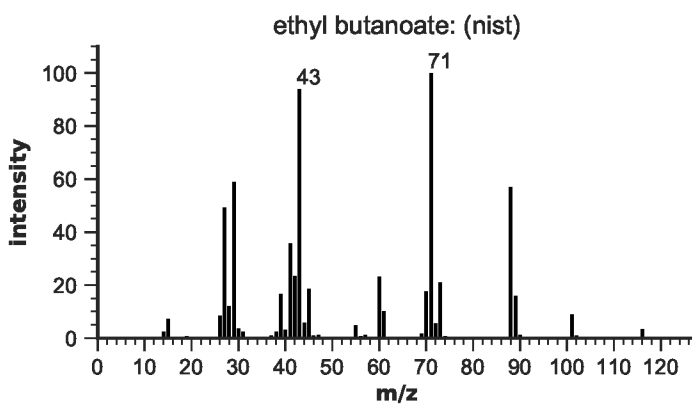
Figure S93: EIMS for ethyl butanoate
