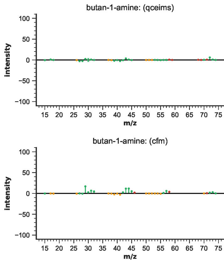
Figure S38: EIMS differences for butan-1-amine
