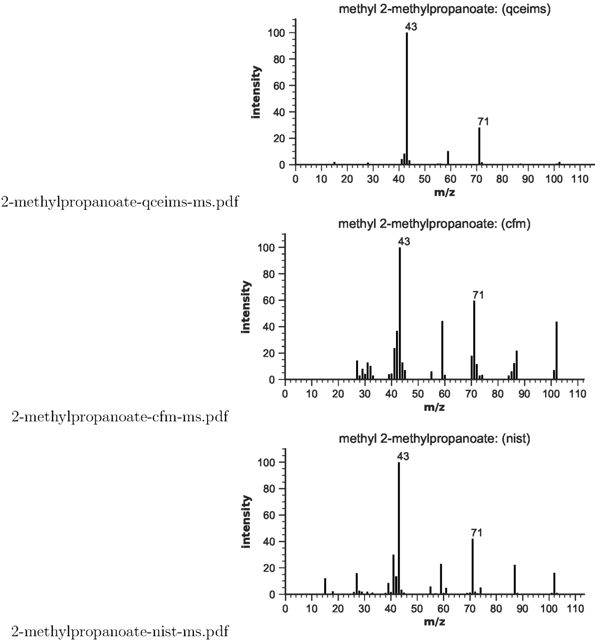
Figure S83: EIMS for methyl 2-methylpropanoate
