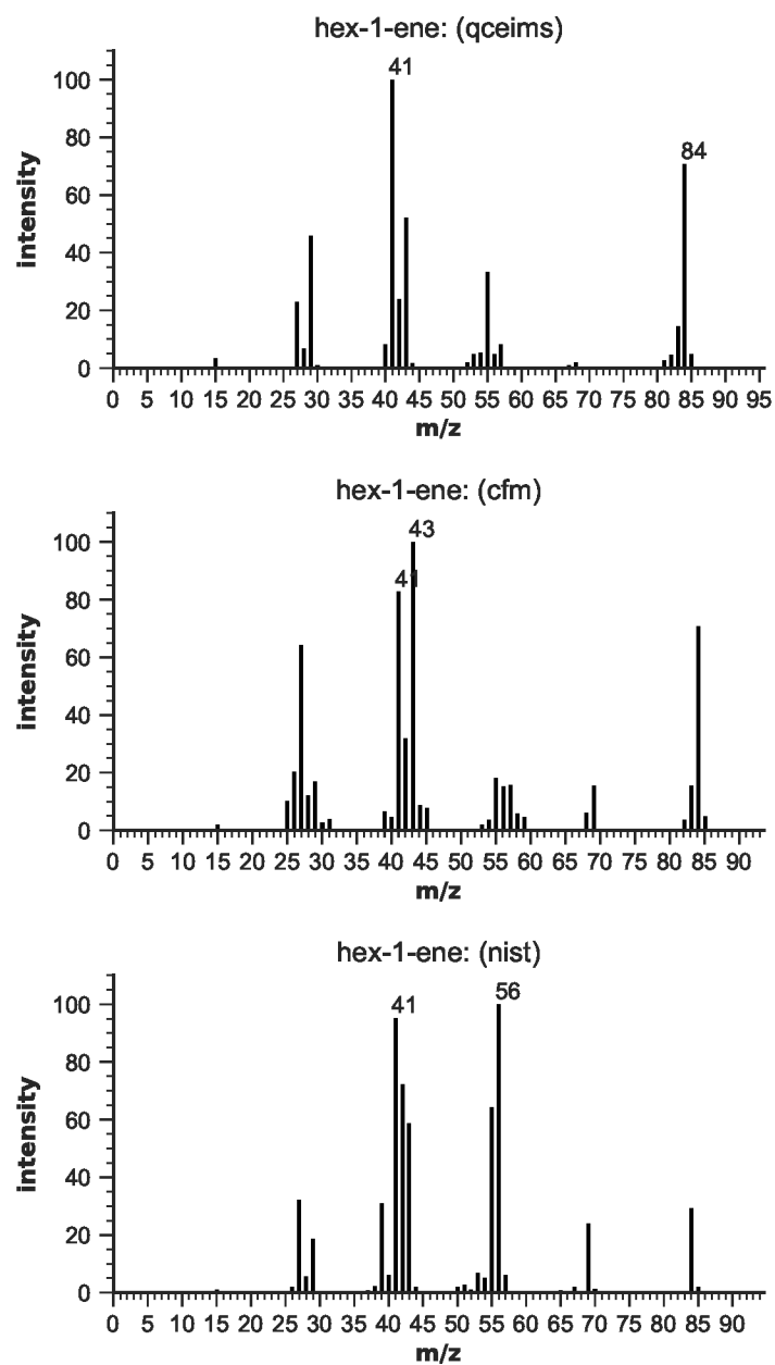
Figure S27: EIMS for hex-1-ene
