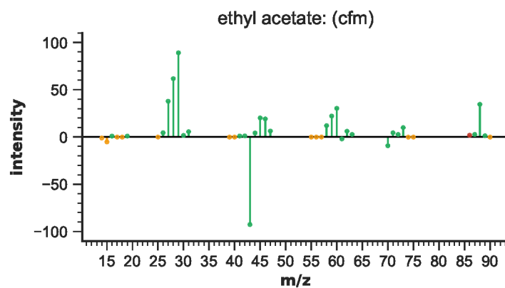
Figure S76: EIMS differences for ethyl acetate
