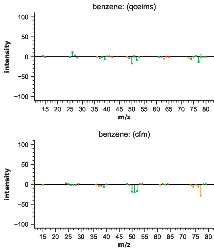
Figure S46: EIMS differences for benzene
