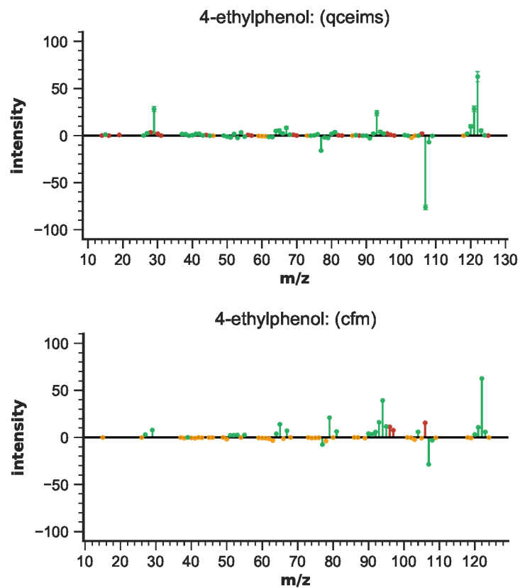
Figure S112: EIMS differences for 4-ethylphenol
