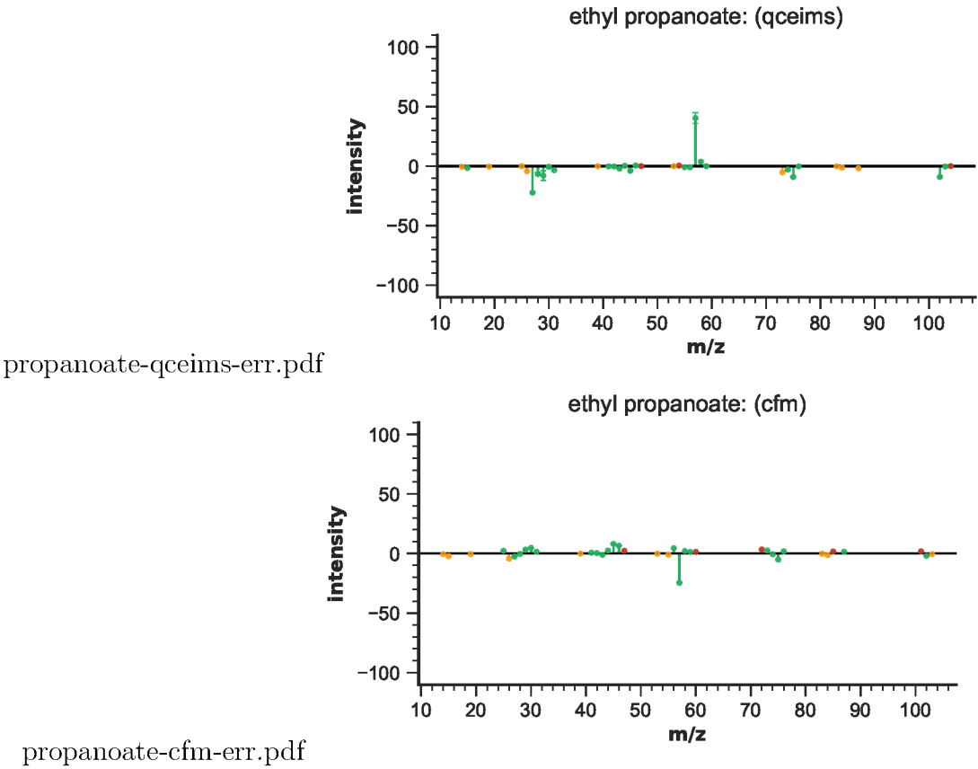
Figure S86: EIMS differences for ethyl propanoate
