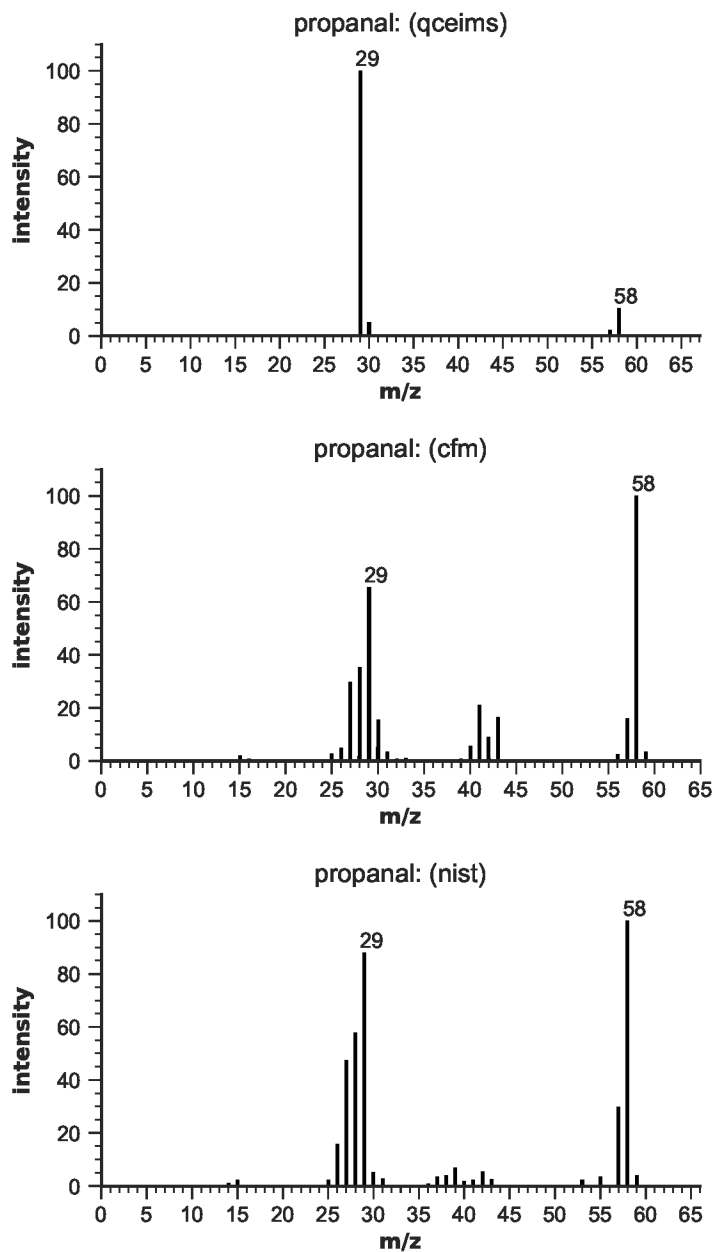
Figure S13: EIMS for propanal
