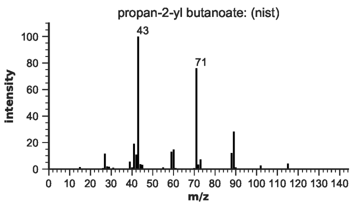
Figure S101: EIMS for propan-2-yl butanoate
