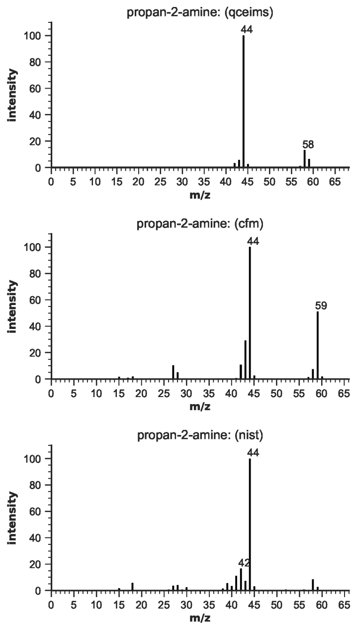
Figure S35: EIMS for propan-2-amine
