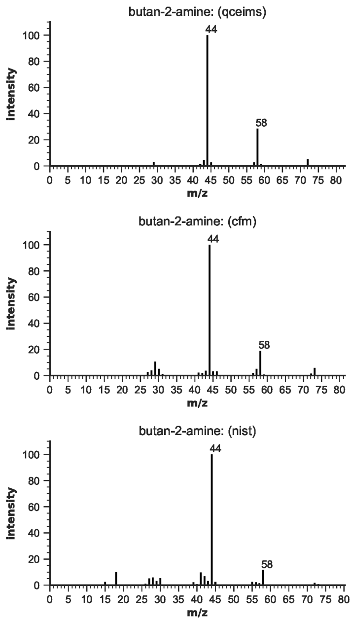
Figure S39: EIMS for butan-2-amine
