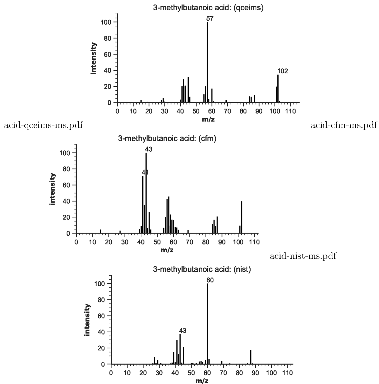
Figure S69: EIMS for 3-methylbutanoic acid
