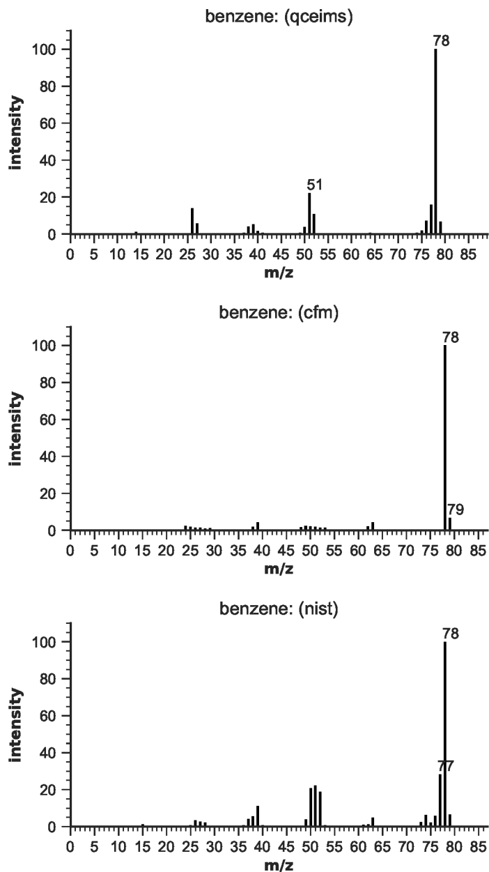
Figure S45: EIMS for benzene
