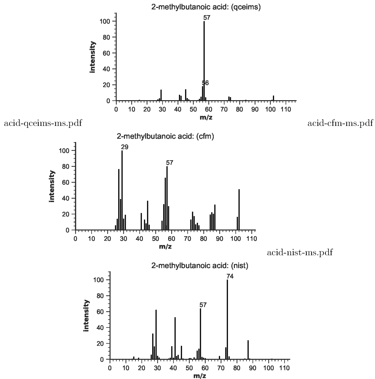
Figure S67: EIMS for 2-methylbutanoic acid
