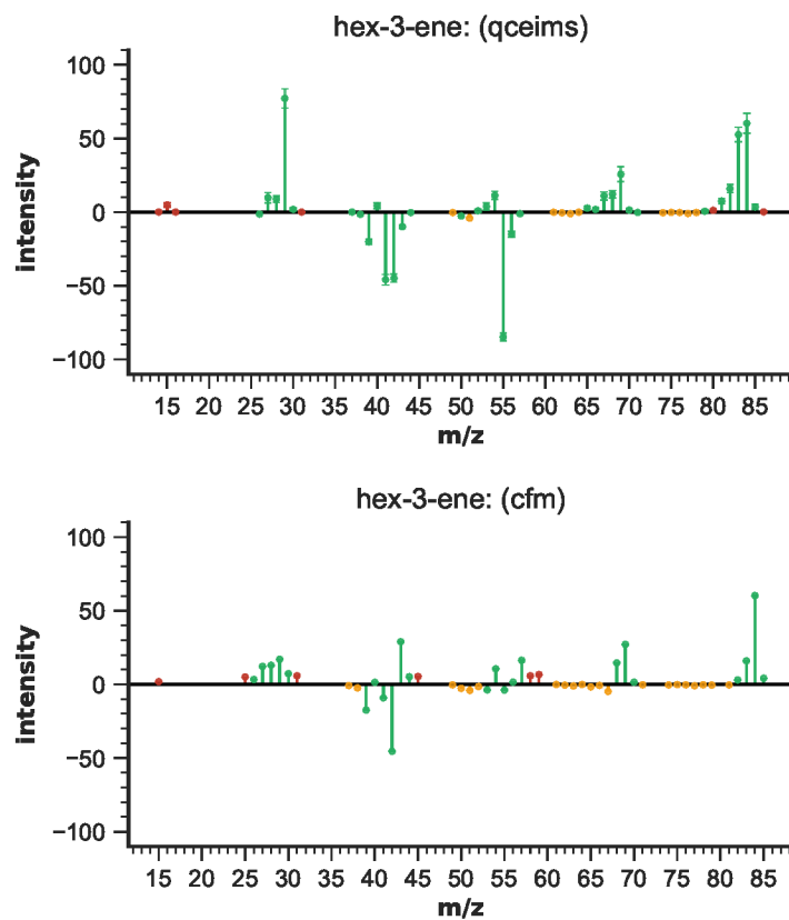
Figure S32: EIMS differences for hex-3-ene
