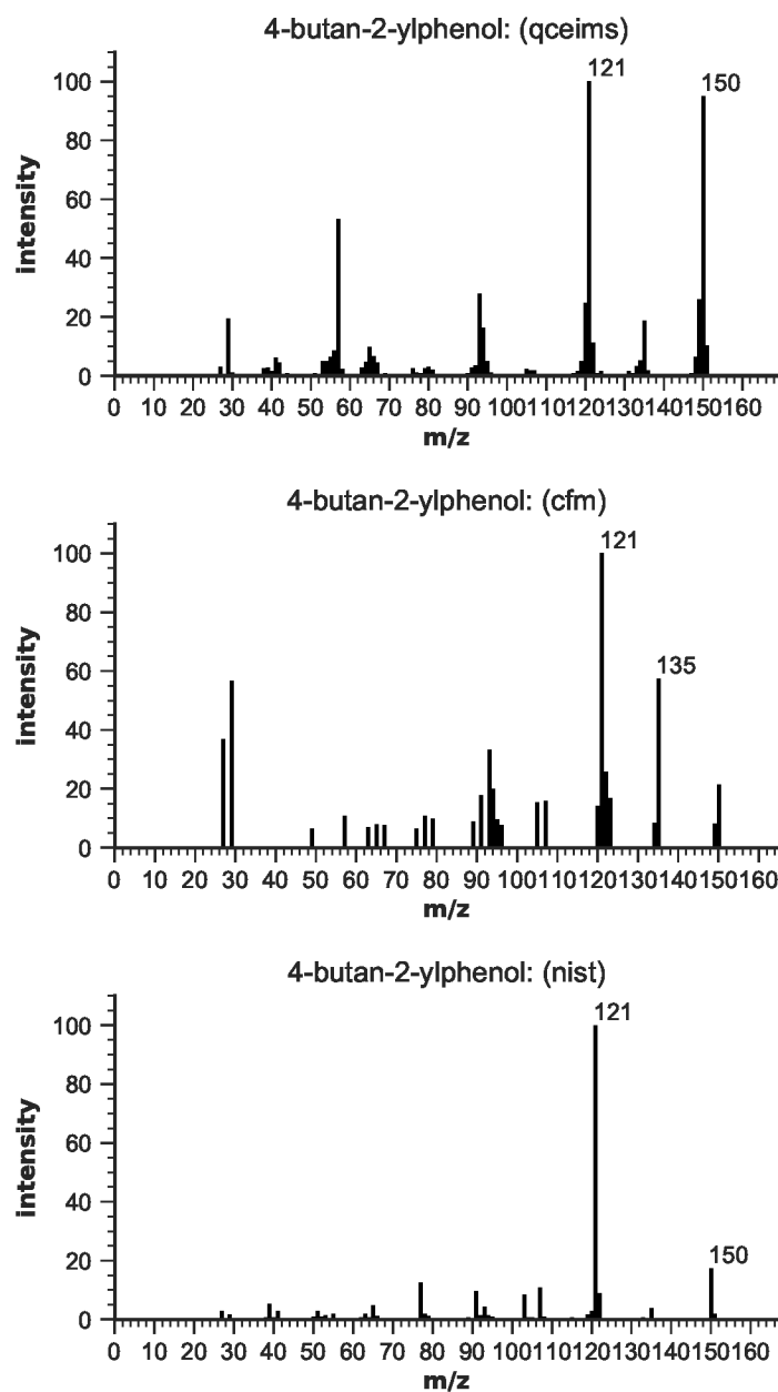
Figure S119: EIMS for 4-butan-2-ylphenol
