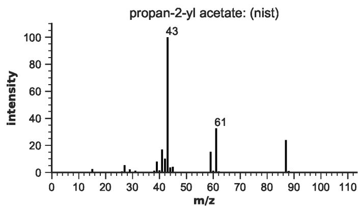
Figure S81: EIMS for propan-2-yl acetate
