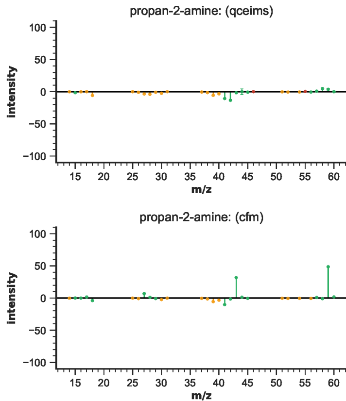
Figure S36: EIMS differences for propan-2-amine
