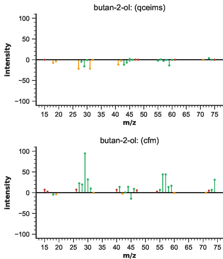
Figure S8: EIMS differences for butan-2-ol
