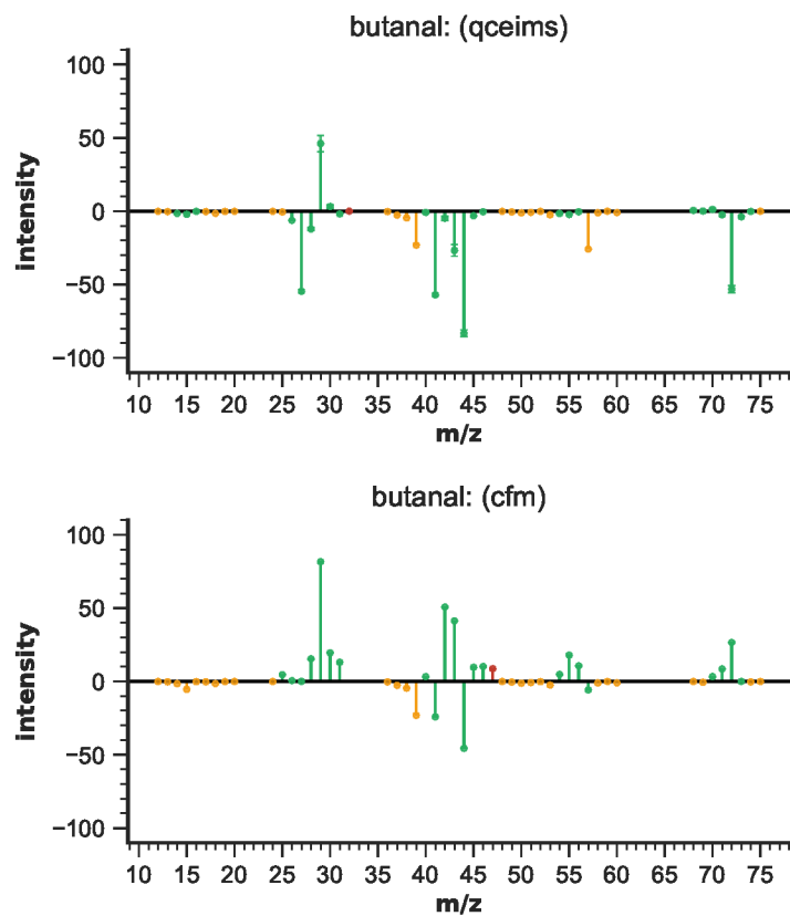
Figure S18: EIMS differences for butanal
