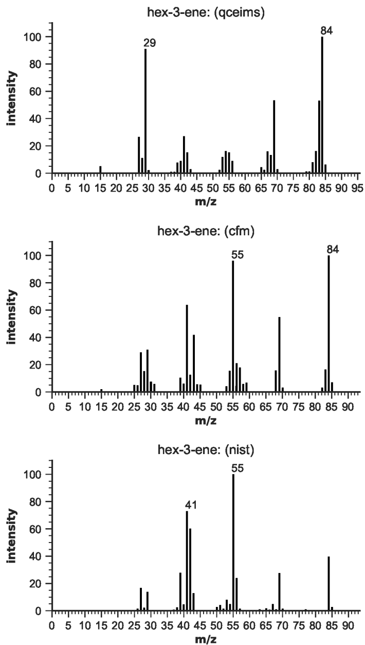
Figure S31: EIMS for hex-3-ene
