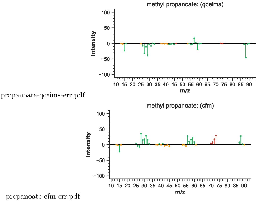
Figure S78: EIMS differences for methyl propanoate
