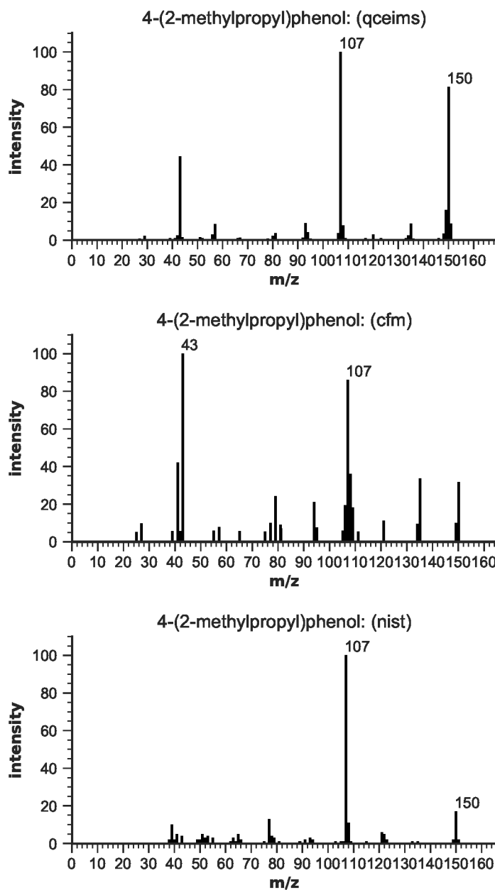
Figure S121: EIMS for 4-(2-methylpropyl)phenol
