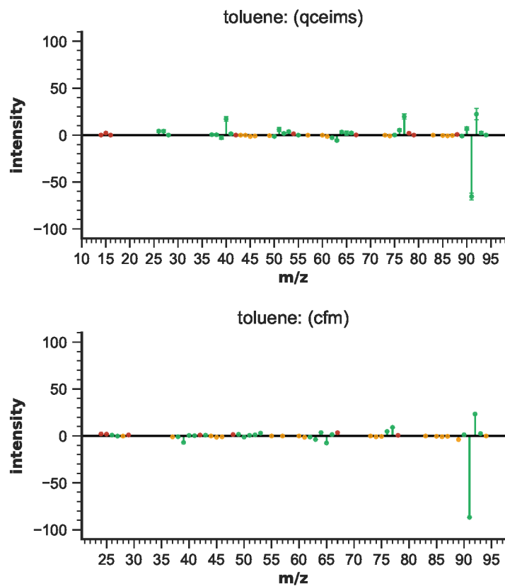
Figure S48: EIMS differences for toluene
