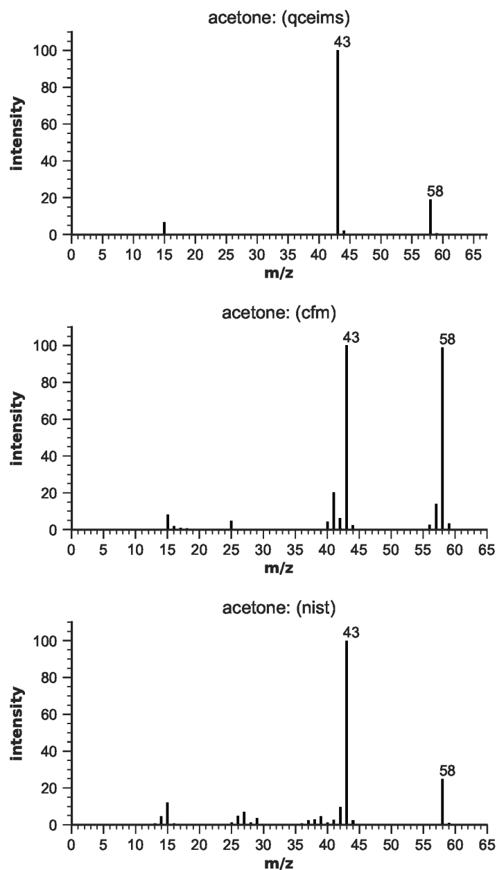
Figure S103: EIMS for acetone
