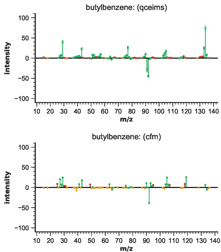
Figure S56: EIMS differences for butylbenzene
