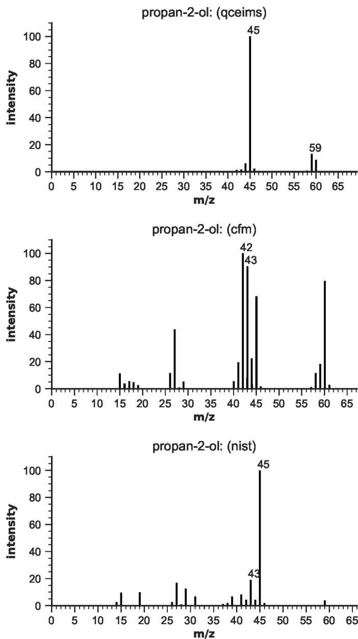
Figure S3: EIMS for propan-2-ol
