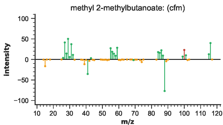
Figure S96: EIMS differences for methyl 2-methylbutanoate
