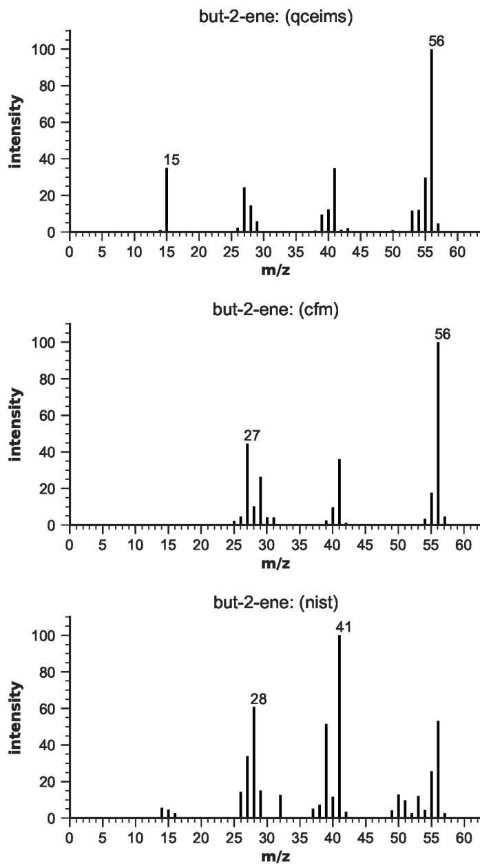
Figure S21: EIMS for but-2-ene
