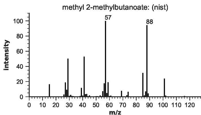
Figure S95: EIMS for methyl 2-methylbutanoate
