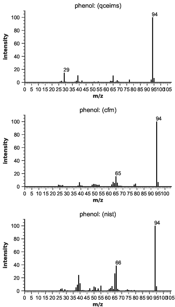
Figure S107: EIMS for phenol
