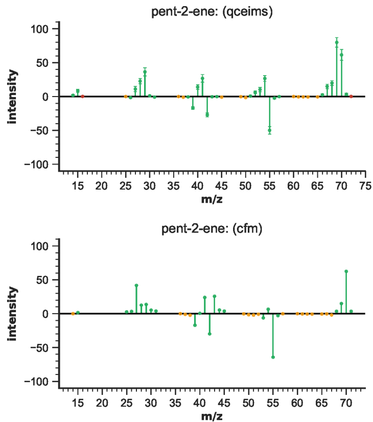
Figure S26: EIMS differences for pent-2-ene
