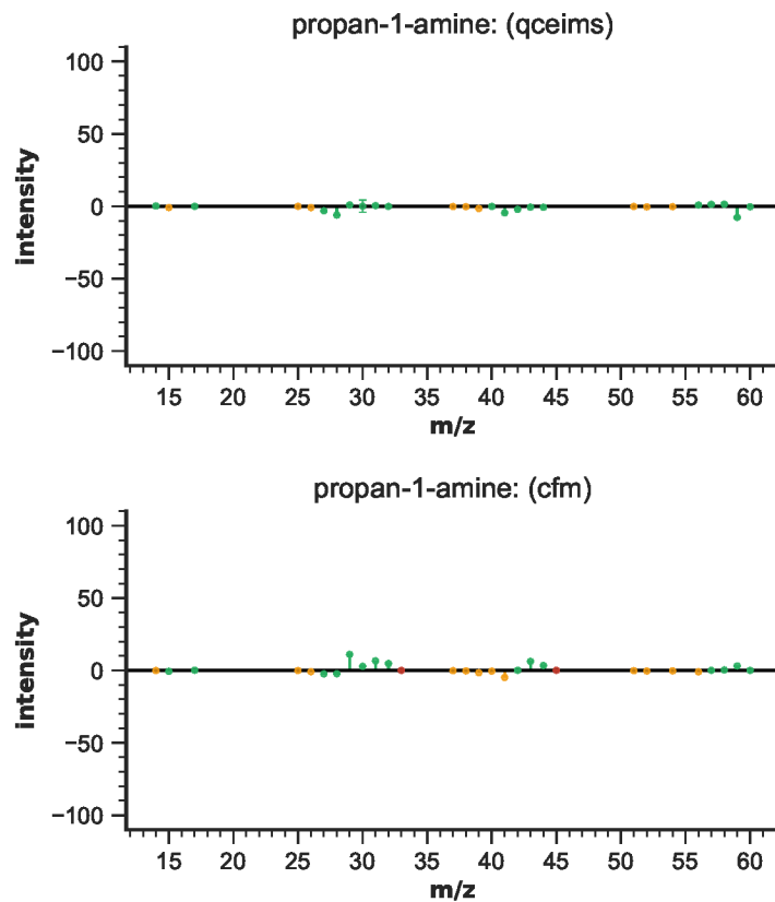
Figure S34: EIMS differences for propan-1-amine
