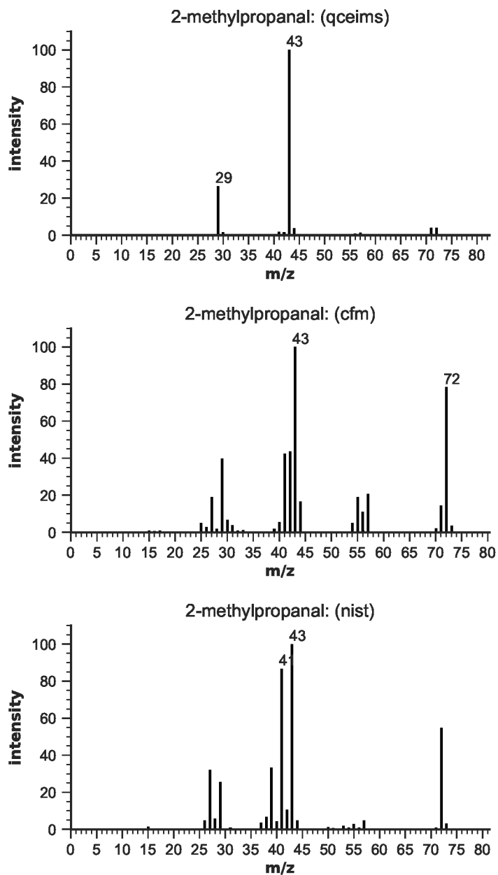
Figure S15: EIMS for 2-methylpropanal
