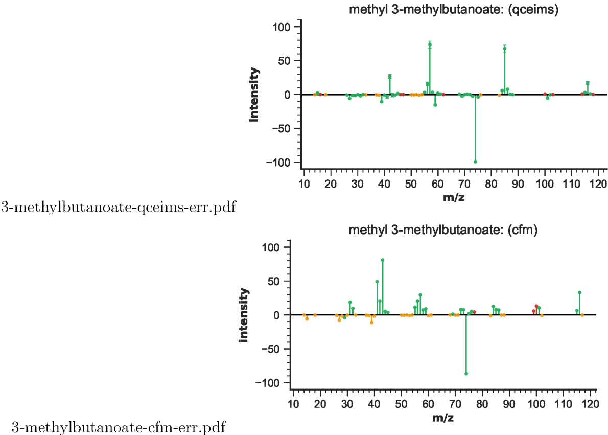
Figure S98: EIMS differences for methyl 3-methylbutanoate
