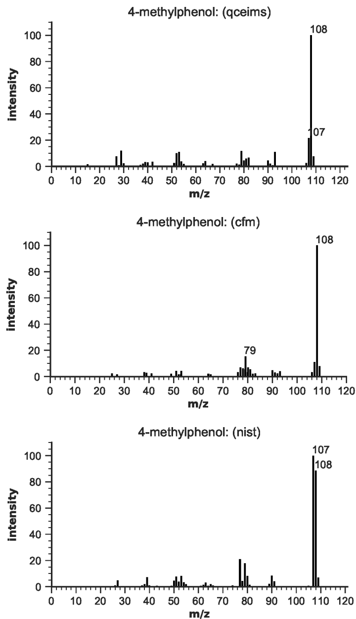
Figure S109: EIMS for 4-methylphenol
