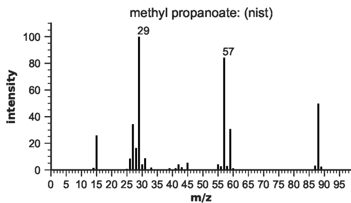
Figure S77: EIMS for methyl propanoate
