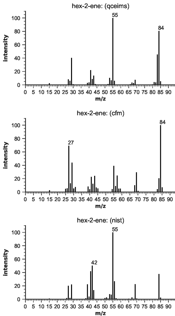
Figure S29: EIMS for hex-2-ene
