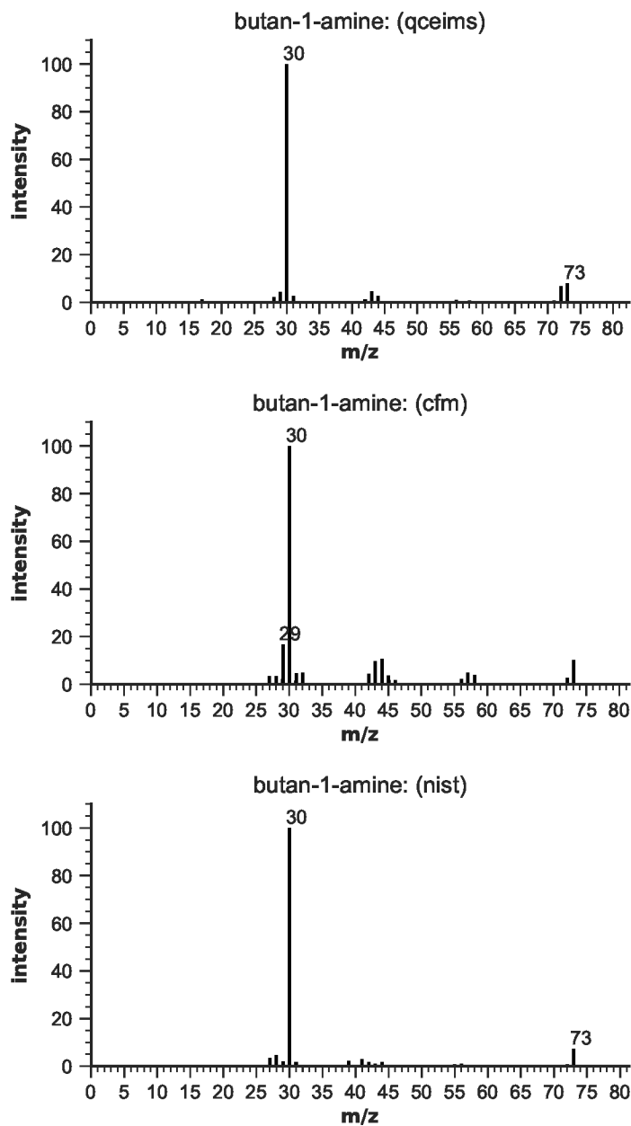
Figure S37: EIMS for butan-1-amine
