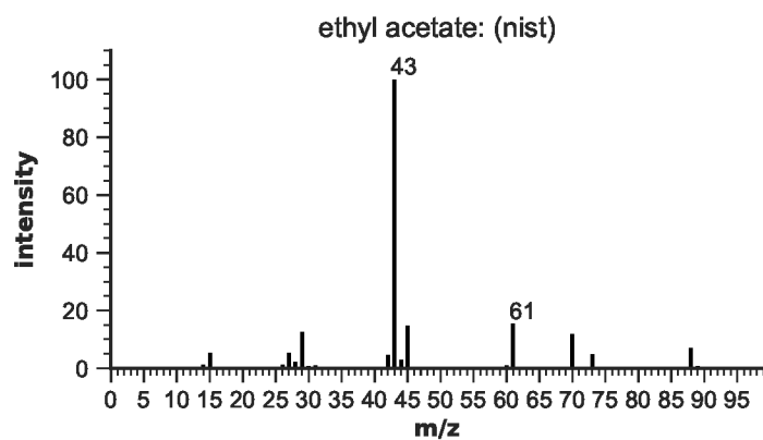
Figure S75: EIMS for ethyl acetate
