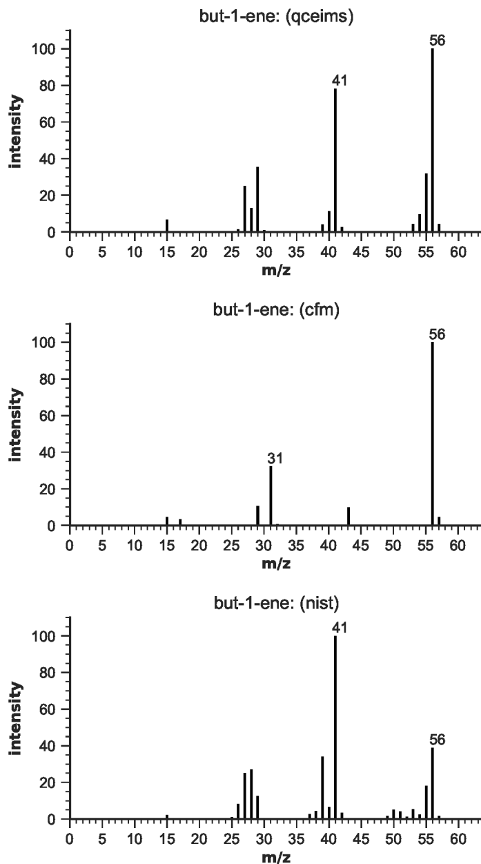
Figure S19: EIMS for but-1-ene
