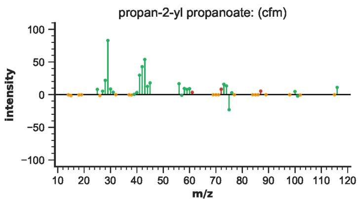
Figure S92: EIMS differences for propan-2-yl propanoate
