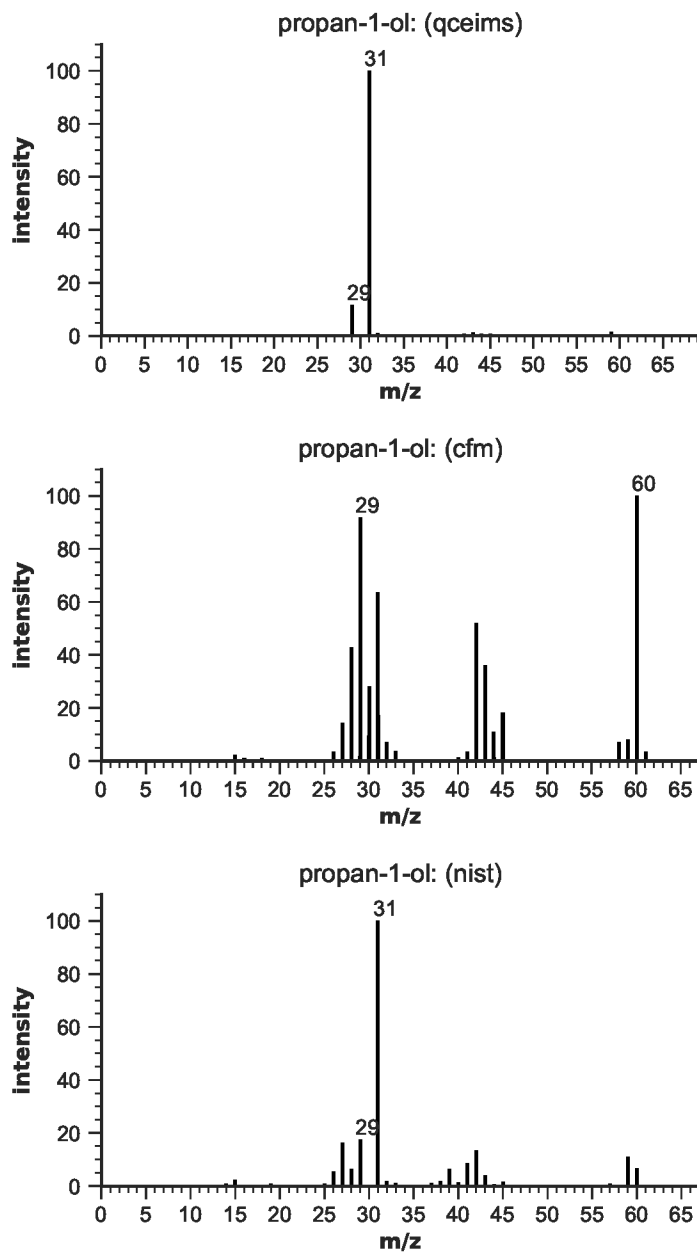
Figure S1: EIMS for propan-1-ol
