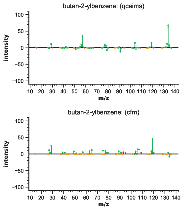
Figure S58: EIMS differences for butan-2-ylbenzene
