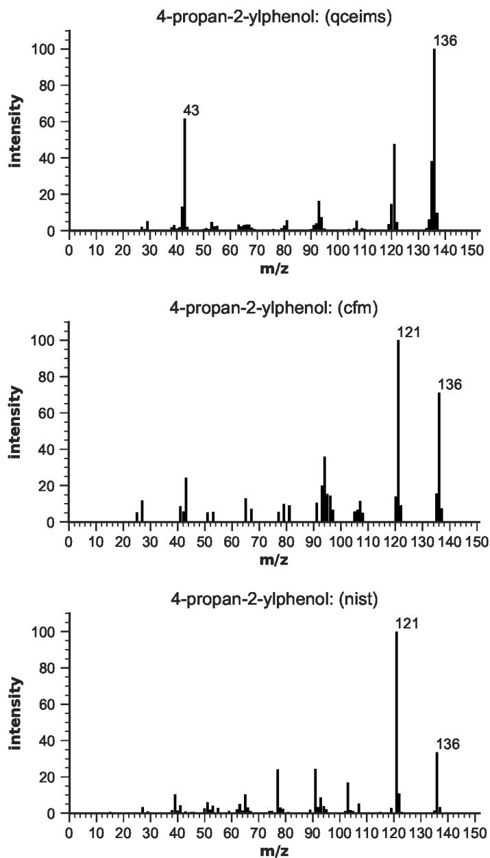
Figure S115: EIMS for 4-propan-2-ylphenol
