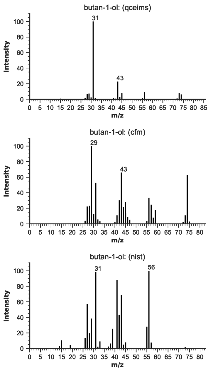
Figure S5: EIMS for butan-1-ol
