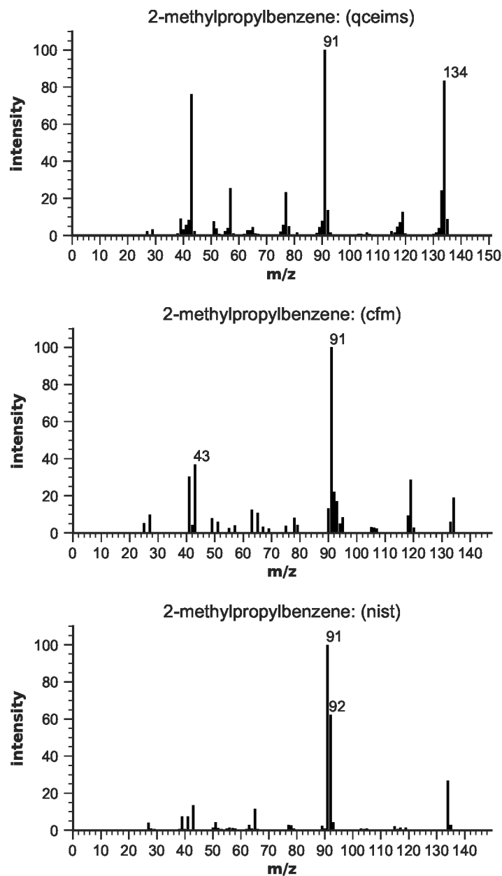
Figure S59: EIMS for 2-methylpropylbenzene
