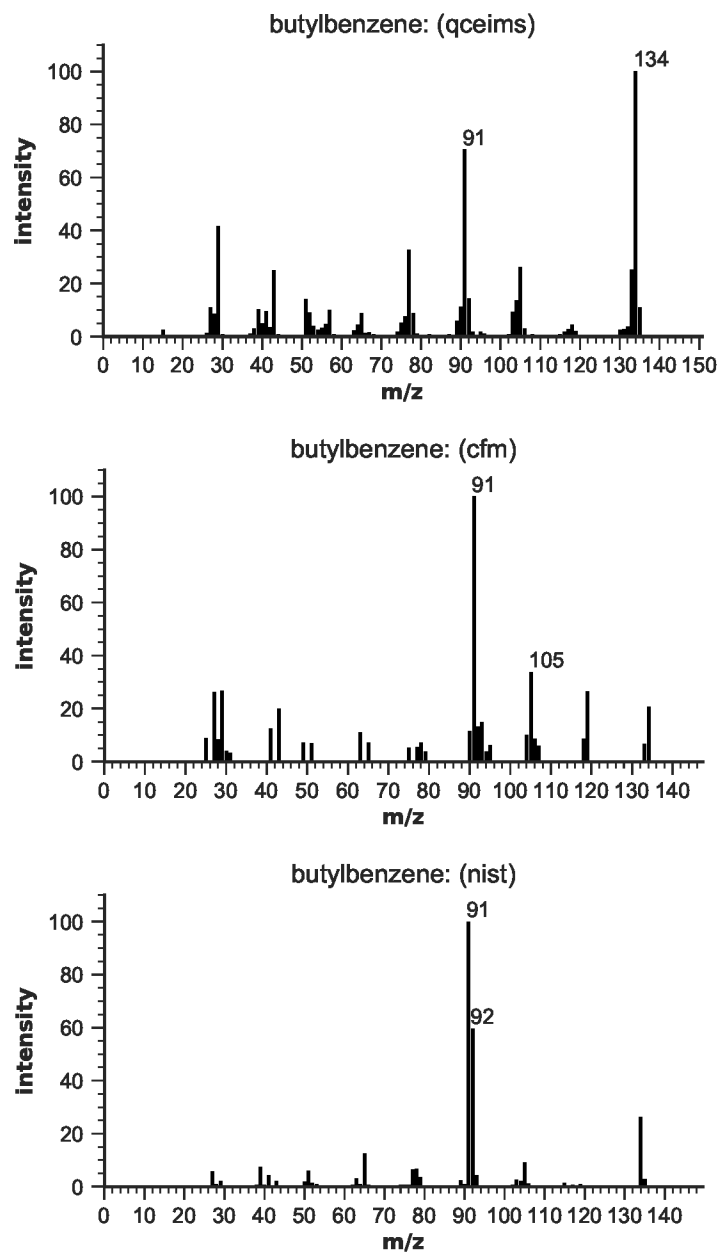
Figure S55: EIMS for butylbenzene
