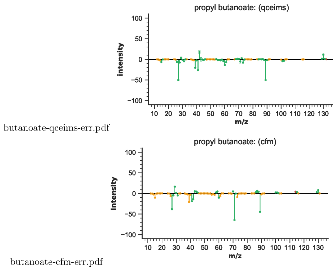
Figure S100: EIMS differences for propyl butanoate
