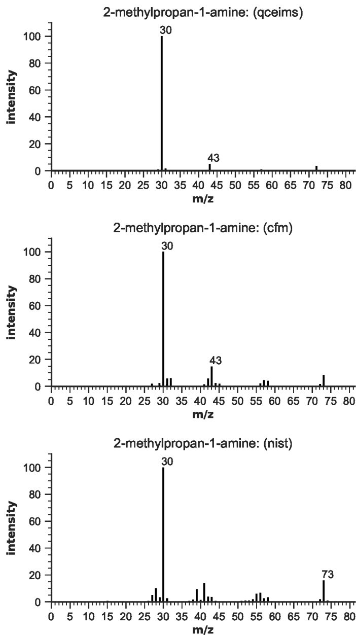
Figure S41: EIMS for 2-methylpropan-1-amine
