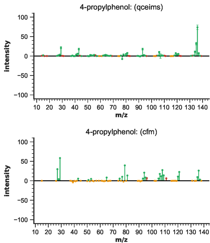
Figure S114: EIMS differences for 4-propylphenol
