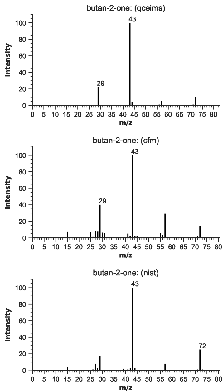
Figure S105: EIMS for butan-2-one
