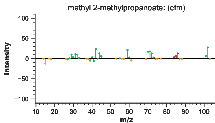
Figure S84: EIMS differences for methyl 2-methylpropanoate
