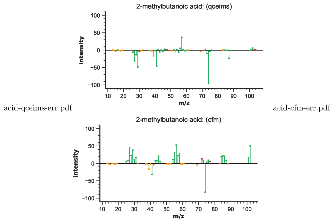
Figure S68: EIMS differences for 2-methylbutanoic acid
