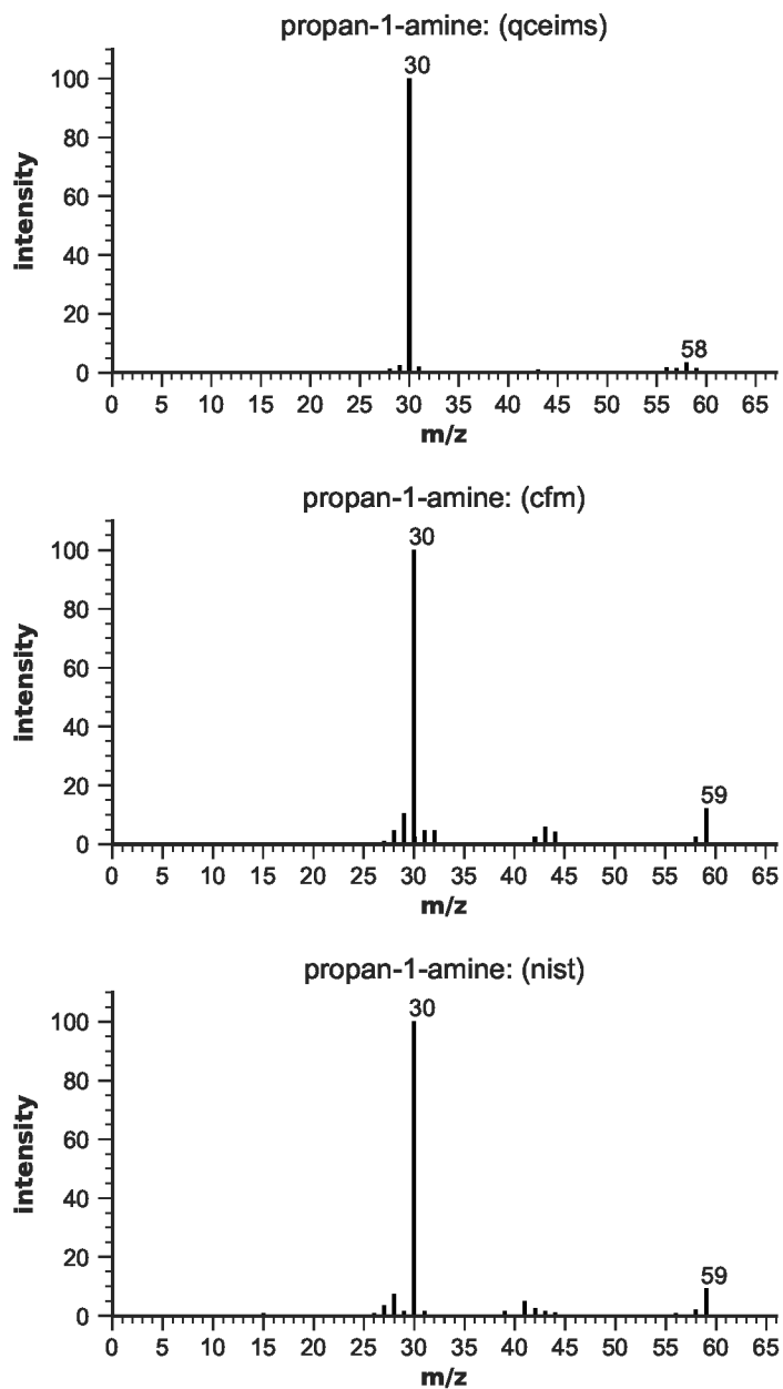
Figure S33: EIMS for propan-1-amine
