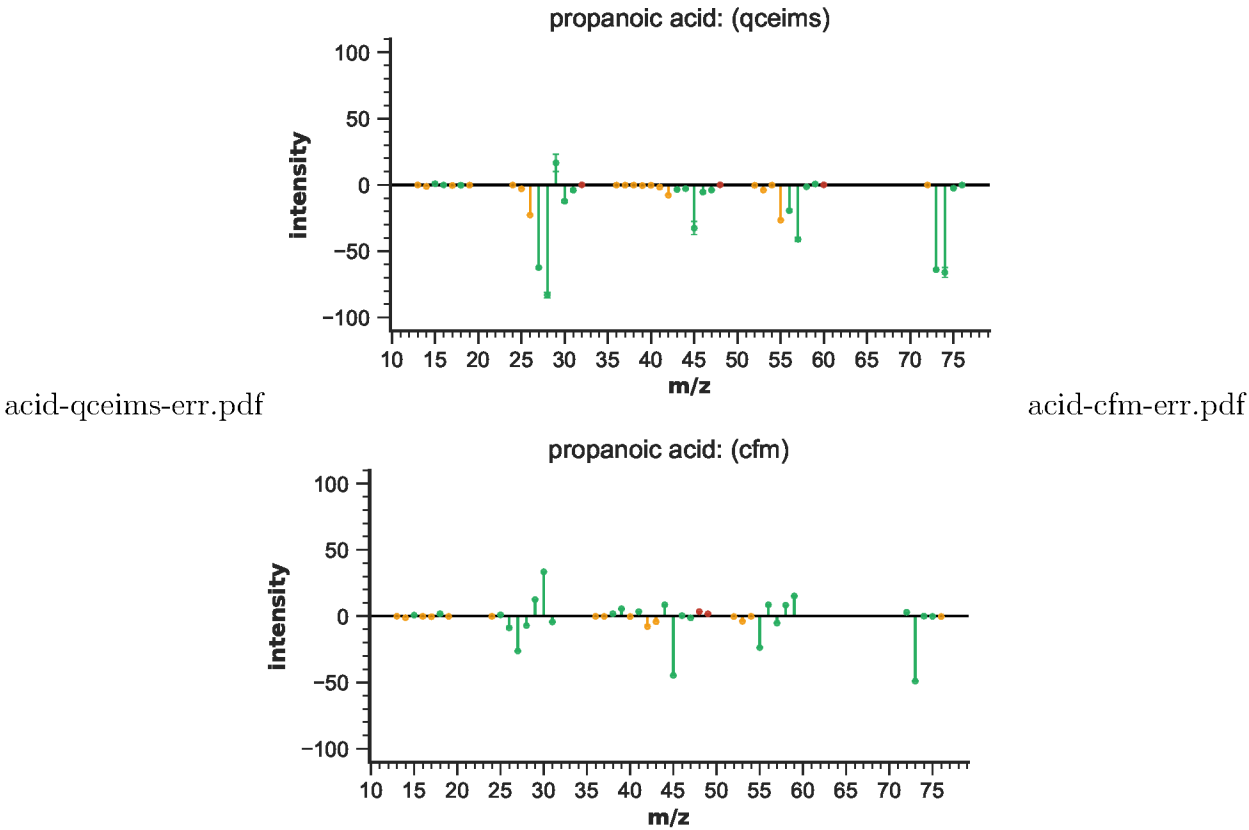
Figure S62: EIMS differences for propanoic acid
