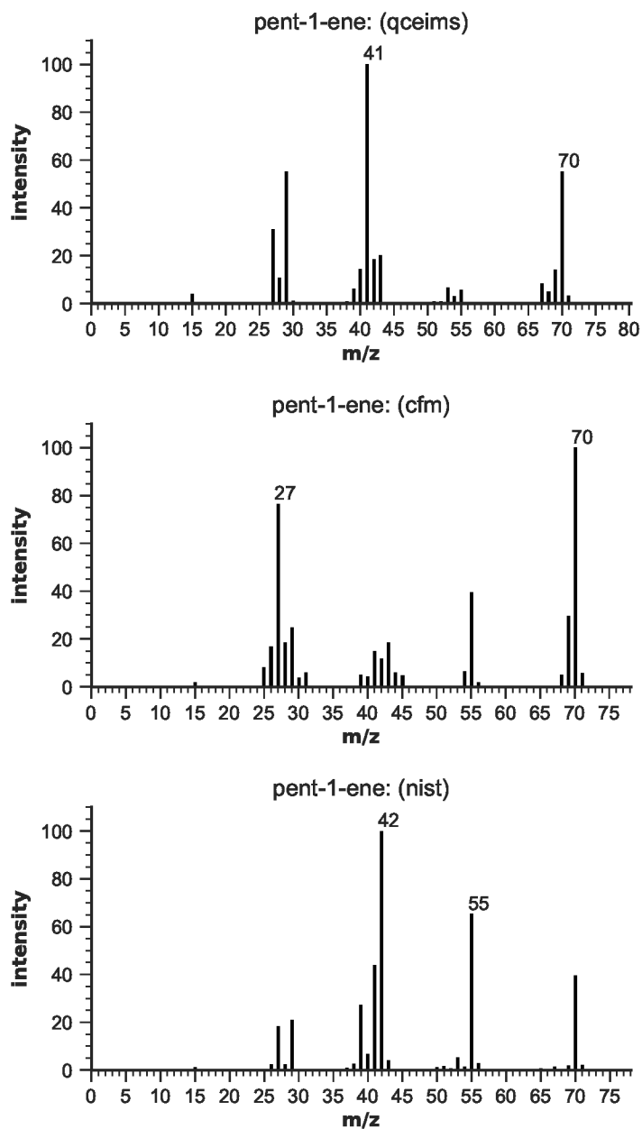
Figure S23: EIMS for pent-1-ene
