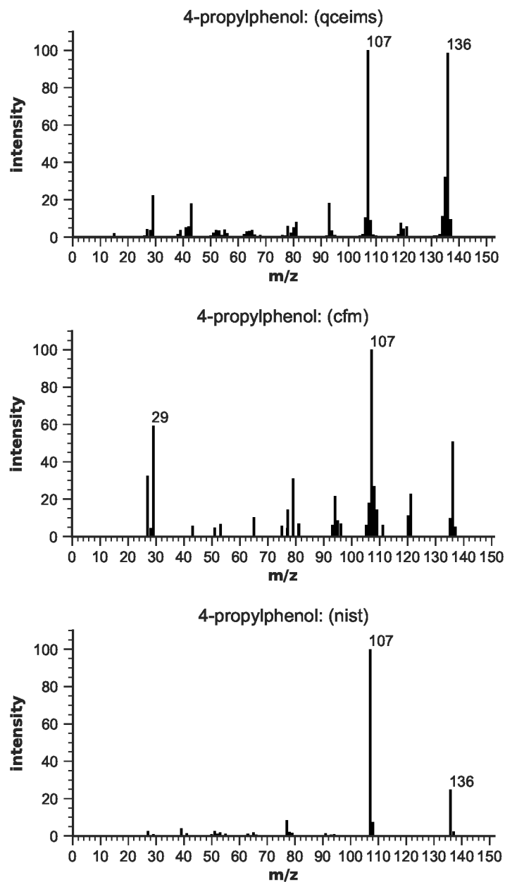
Figure S113: EIMS for 4-propylphenol
