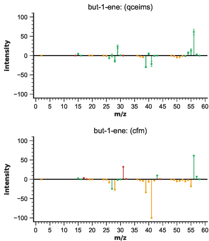
Figure S20: EIMS differences for but-1-ene
