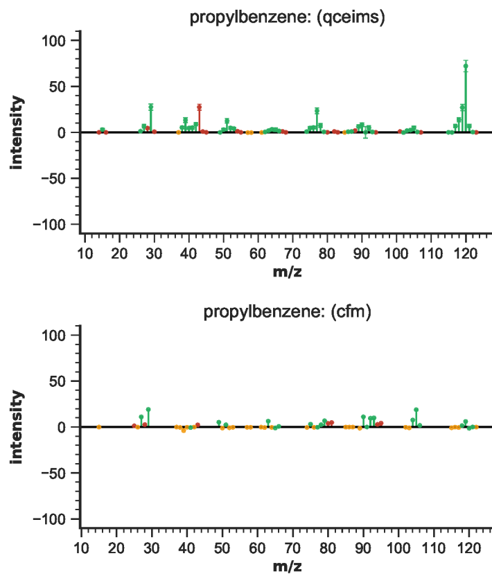
Figure S52: EIMS differences for propylbenzene
