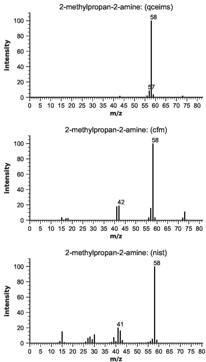
Figure S43: EIMS for 2-methylpropan-2-amine
