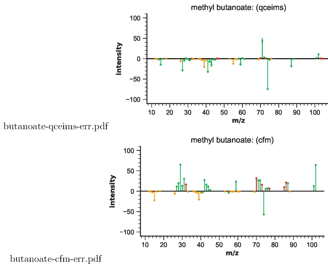
Figure S88: EIMS differences for methyl butanoate
