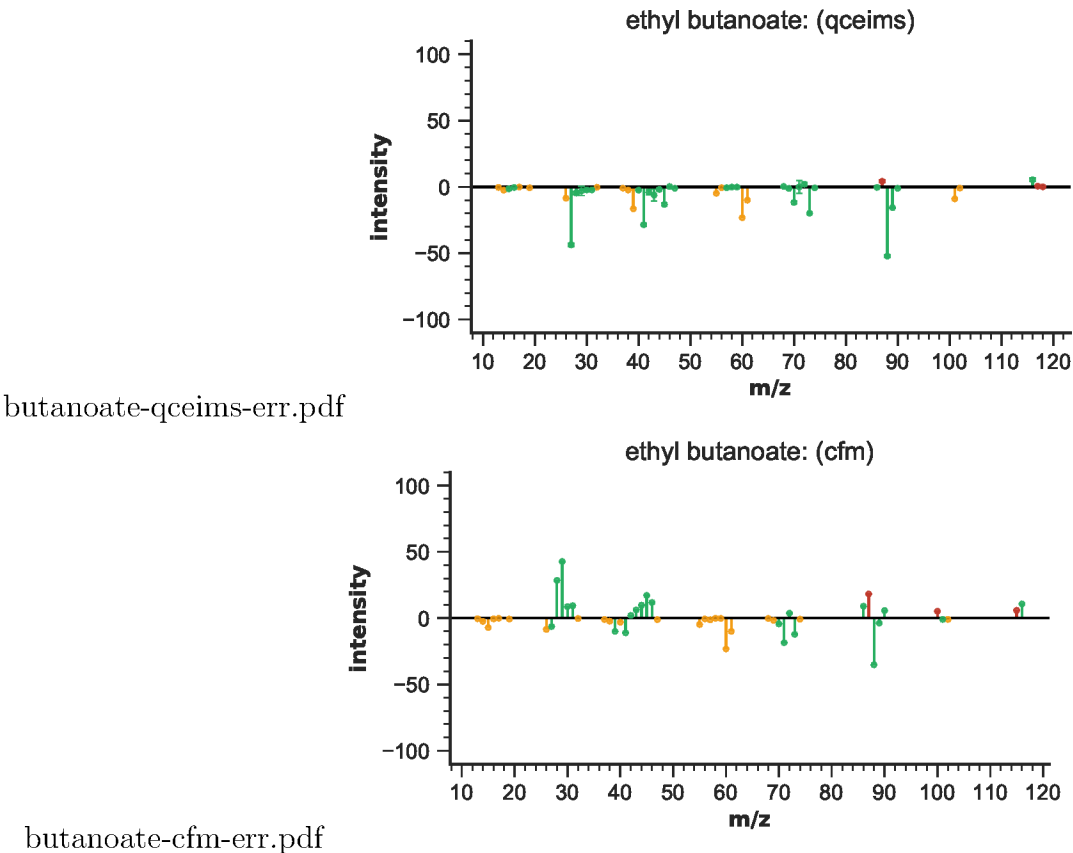
Figure S94: EIMS differences for ethyl butanoate
