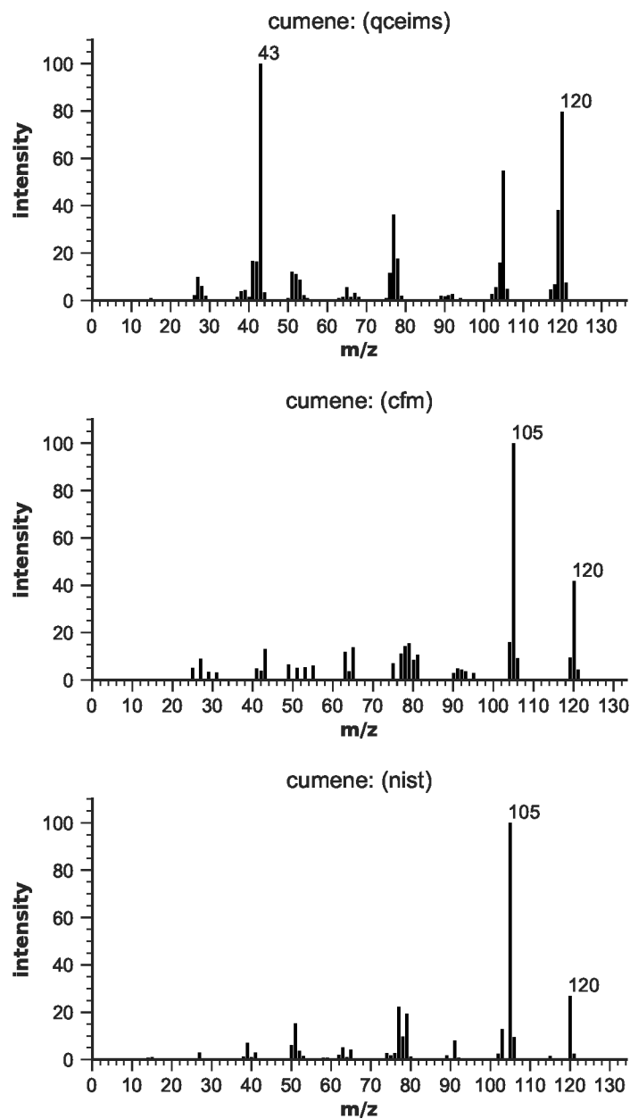
Figure S53: EIMS for cumene
