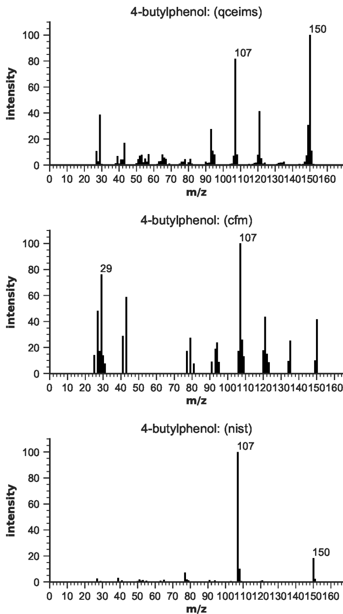
Figure S117: EIMS for 4-butylphenol
