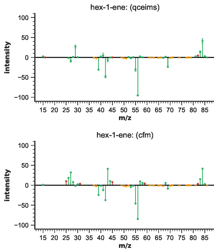
Figure S28: EIMS differences for hex-1-ene
