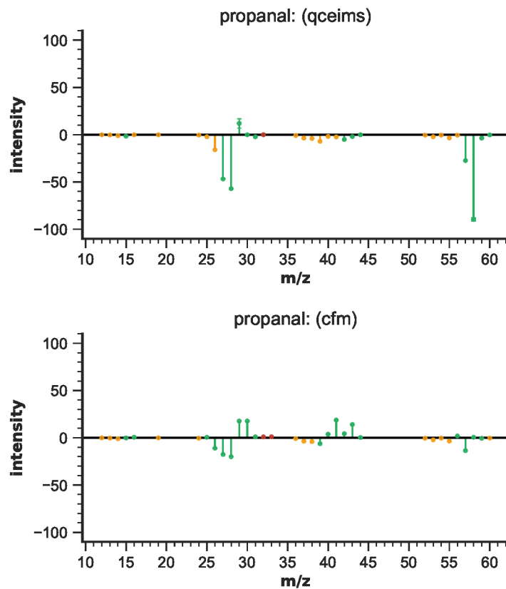
Figure S14: EIMS differences for propanal
