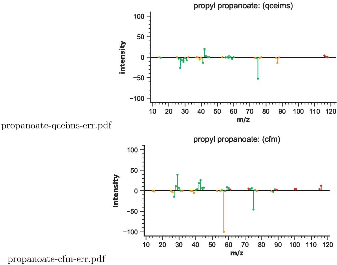
Figure S90: EIMS differences for propyl propanoate
