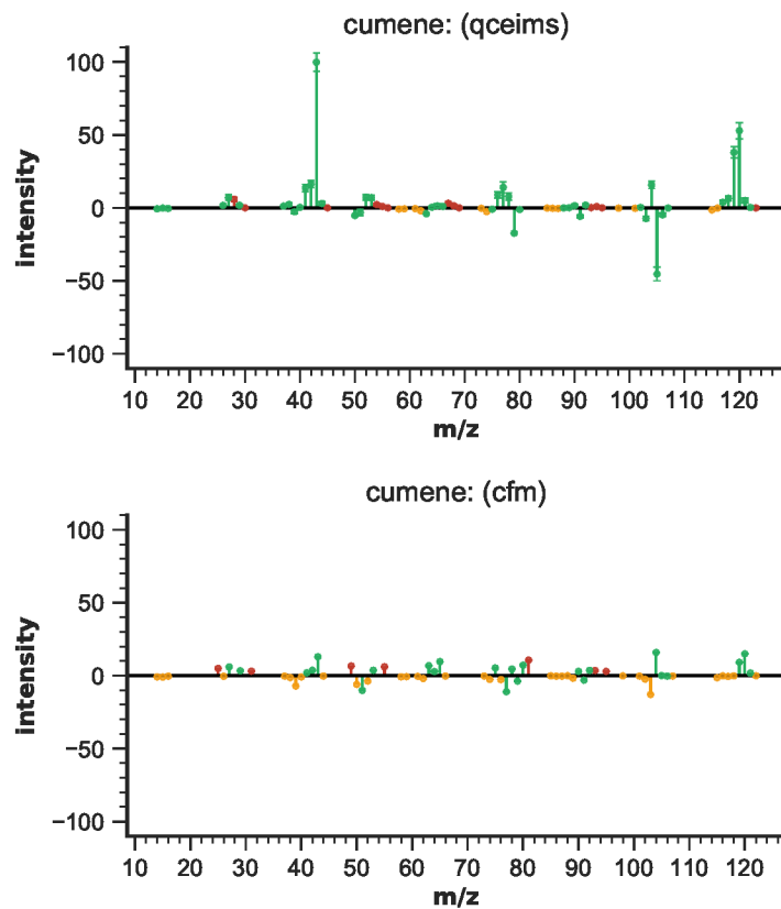
Figure S54: EIMS differences for cumene
