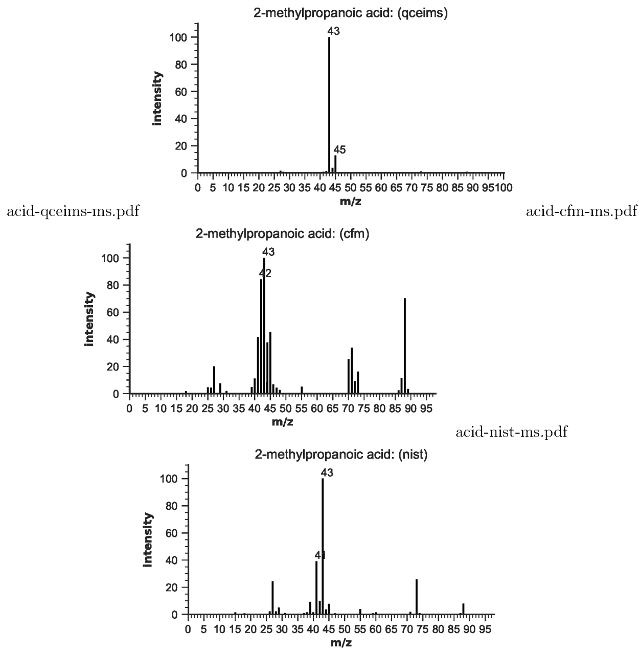
Figure S65: EIMS for 2-methylpropanoic acid
