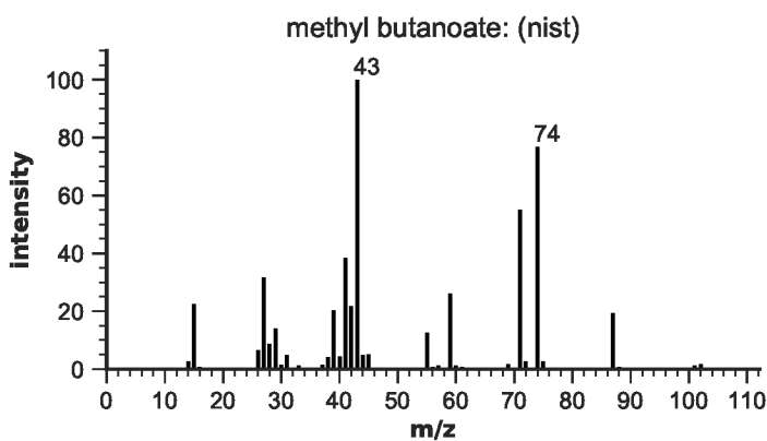
Figure S87: EIMS for methyl butanoate
