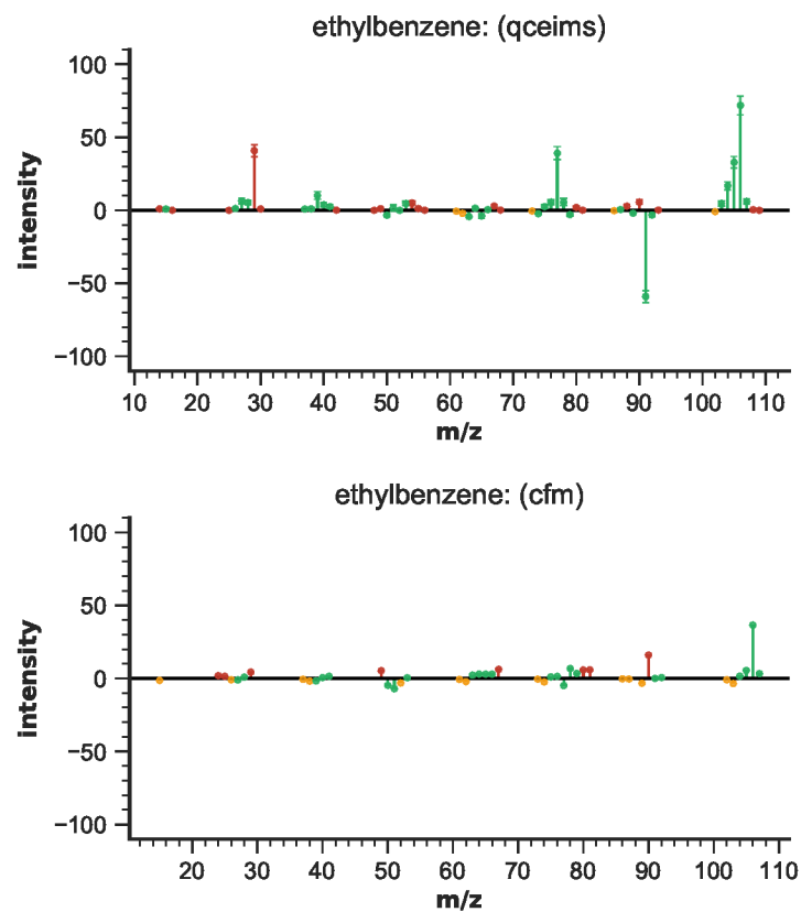
Figure S50: EIMS differences for ethylbenzene
