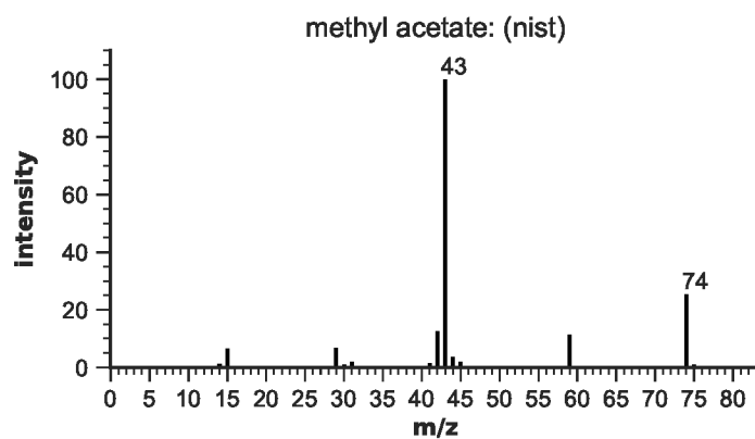
Figure S73: EIMS for methyl acetate
