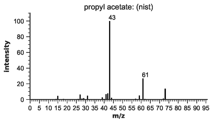
Figure S79: EIMS for propyl acetate
