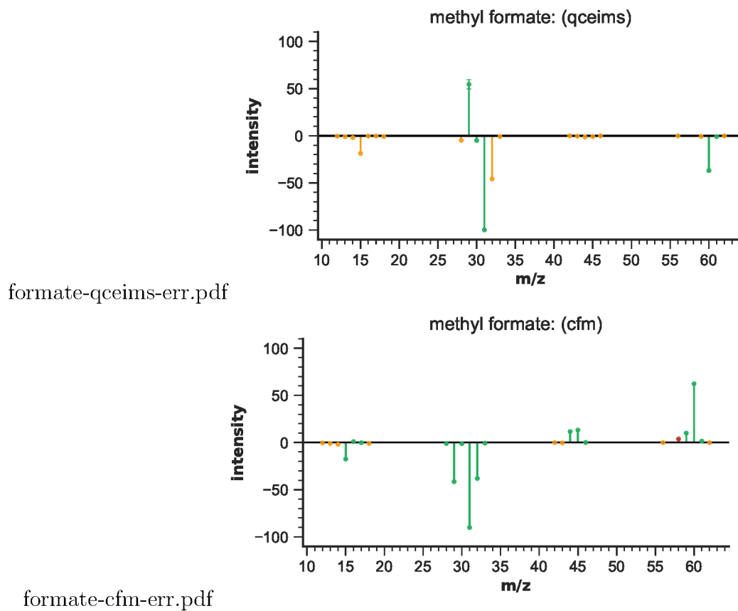
Figure S72: EIMS differences for methyl formate
