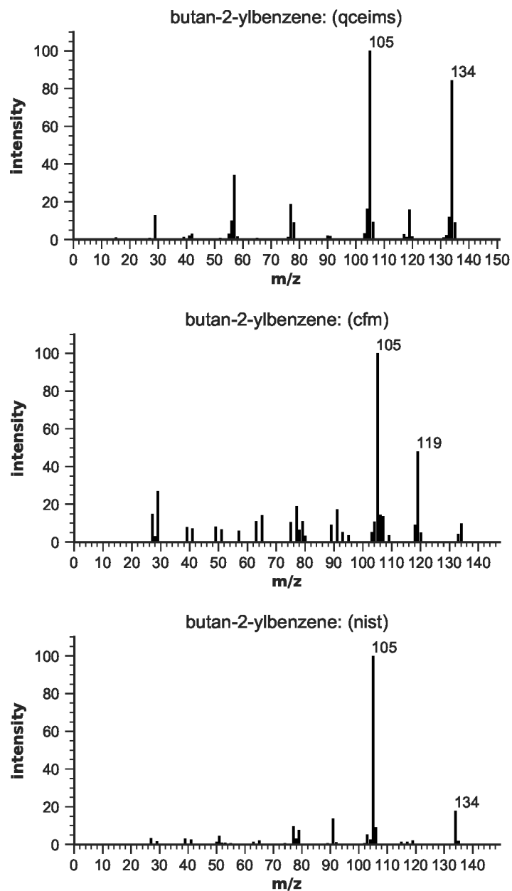
Figure S57: EIMS for butan-2-ylbenzene
