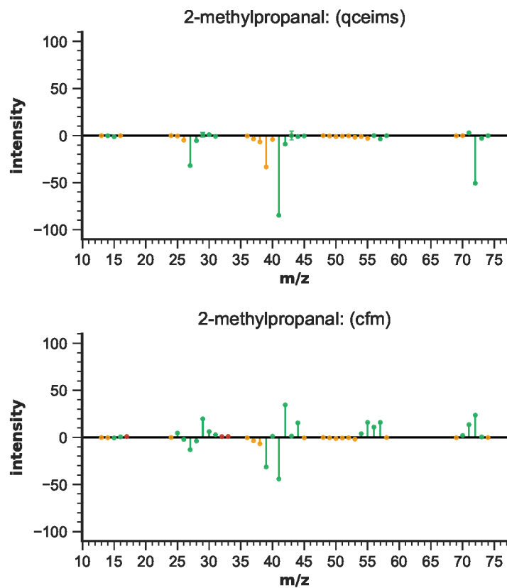
Figure S16: EIMS differences for 2-methylpropanal
