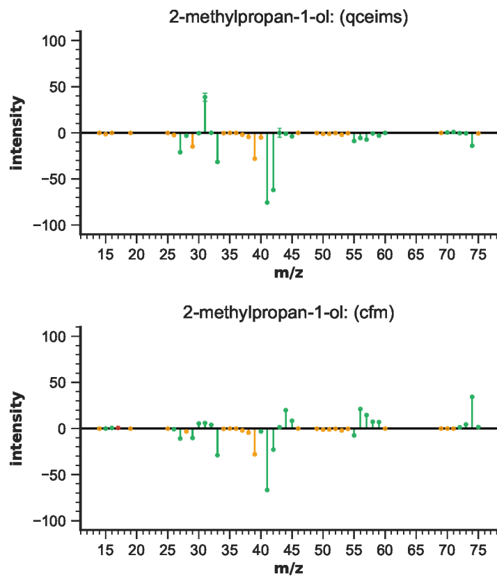
Figure S10: EIMS differences for 2-methylpropan-1-ol
