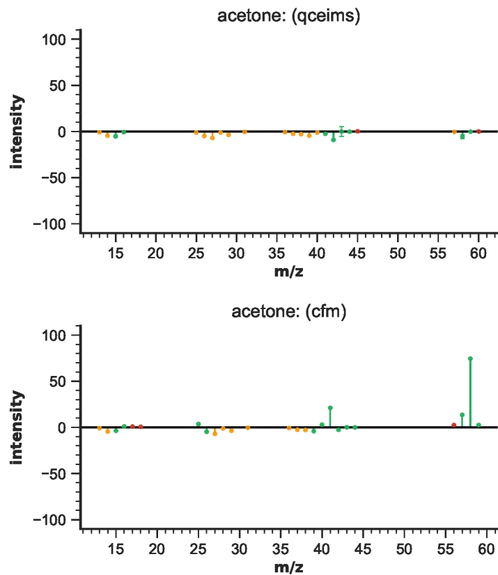
Figure S104: EIMS differences for acetone
