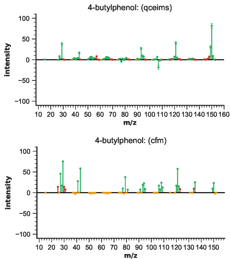
Figure S118: EIMS differences for 4-butylphenol
