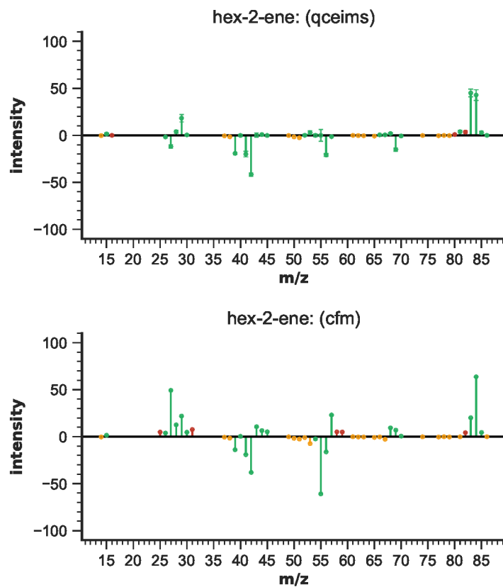
Figure S30: EIMS differences for hex-2-ene
