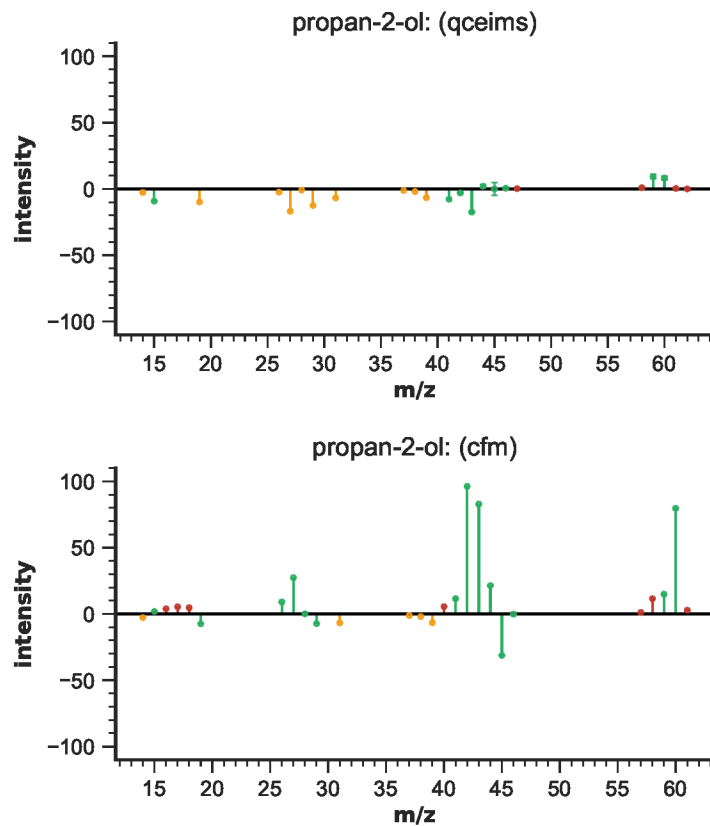
Figure S4: EIMS differences for propan-2-ol
