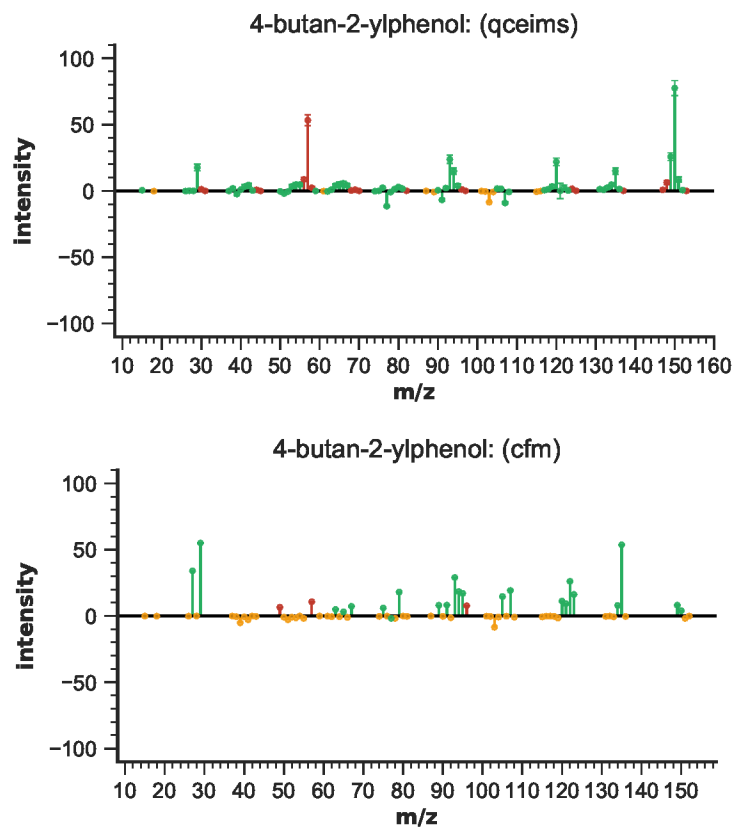
Figure S120: EIMS differences for 4-butan-2-ylphenol
