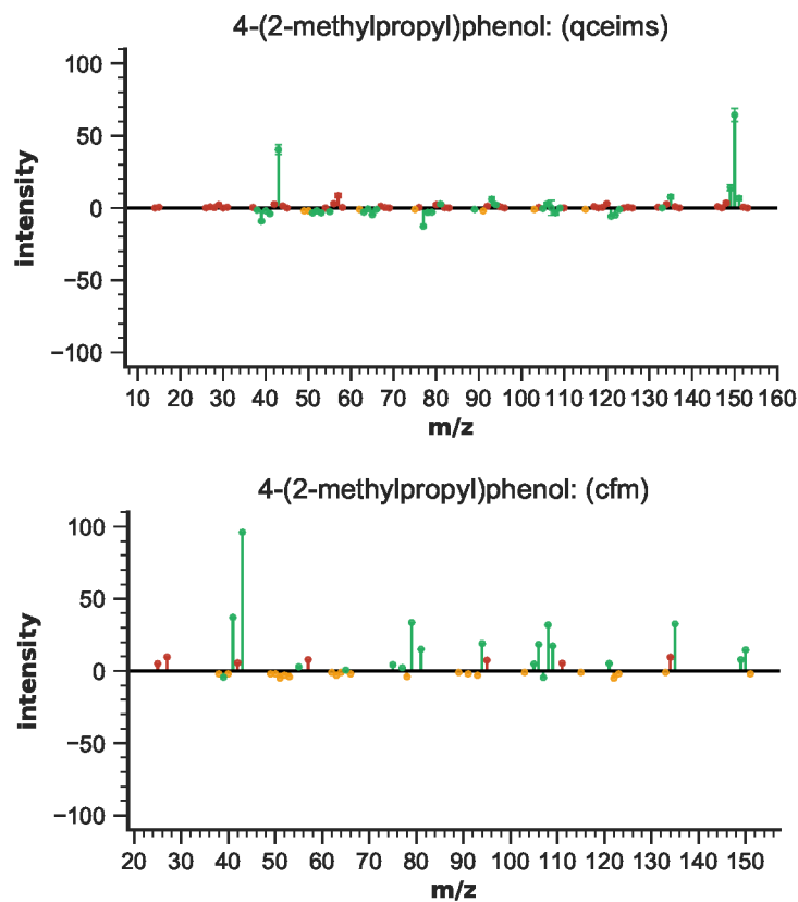
Figure S122: EIMS differences for 4-(2-methylpropyl)phenol
