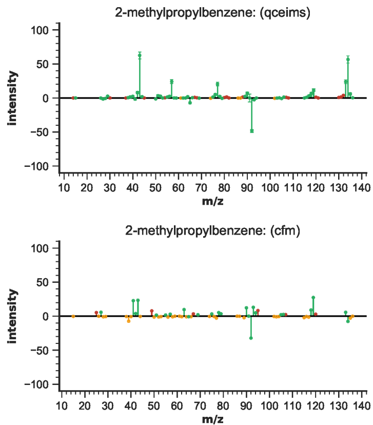
Figure S60: EIMS differences for 2-methylpropylbenzene
