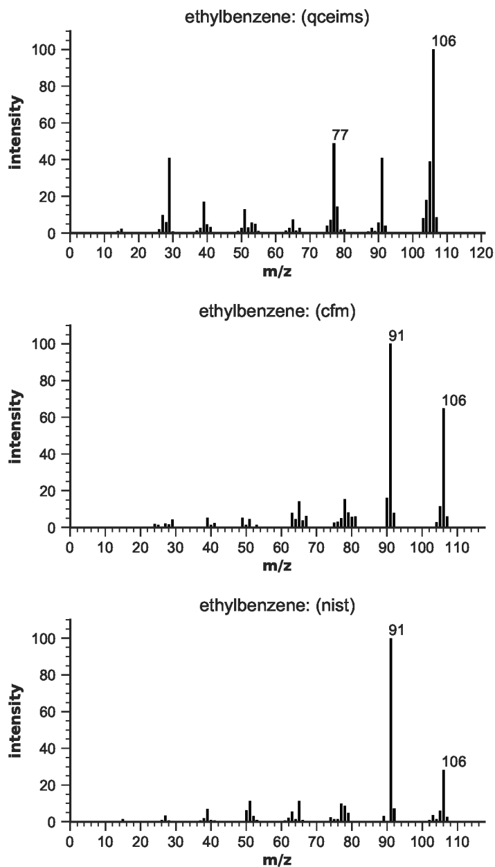
Figure S49: EIMS for ethylbenzene
