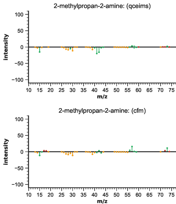
Figure S44: EIMS differences for 2-methylpropan-2-amine
