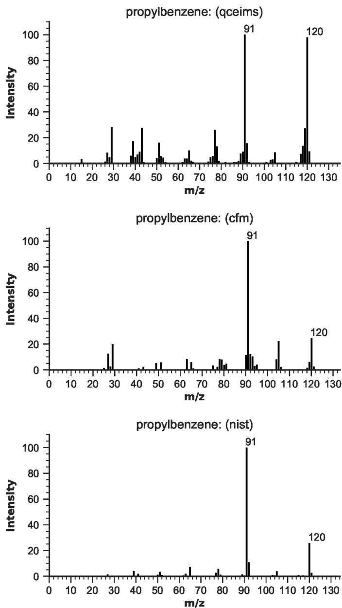
Figure S51: EIMS for propylbenzene
