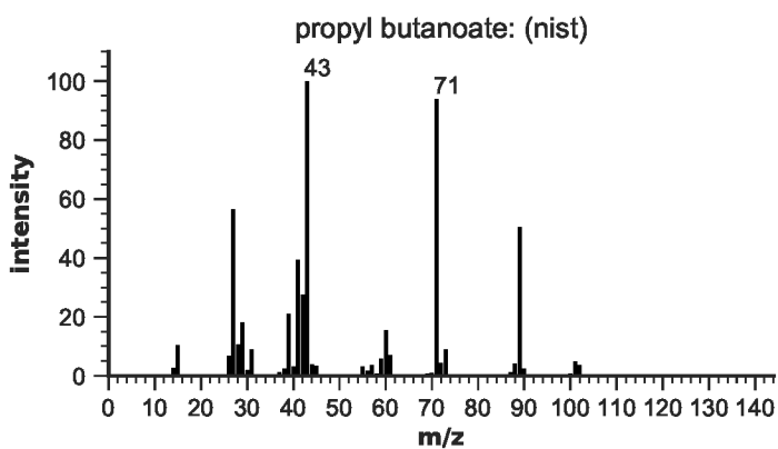
Figure S99: EIMS for propyl butanoate
