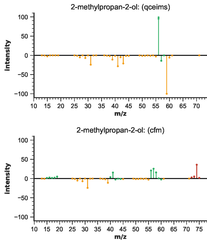
Figure S12: EIMS differences for 2-methylpropan-2-ol
