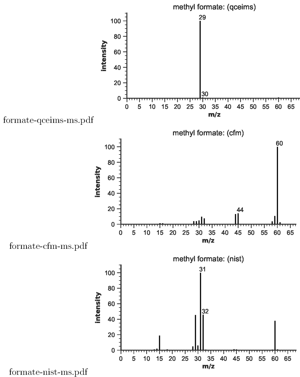
Figure S71: EIMS for methyl formate
