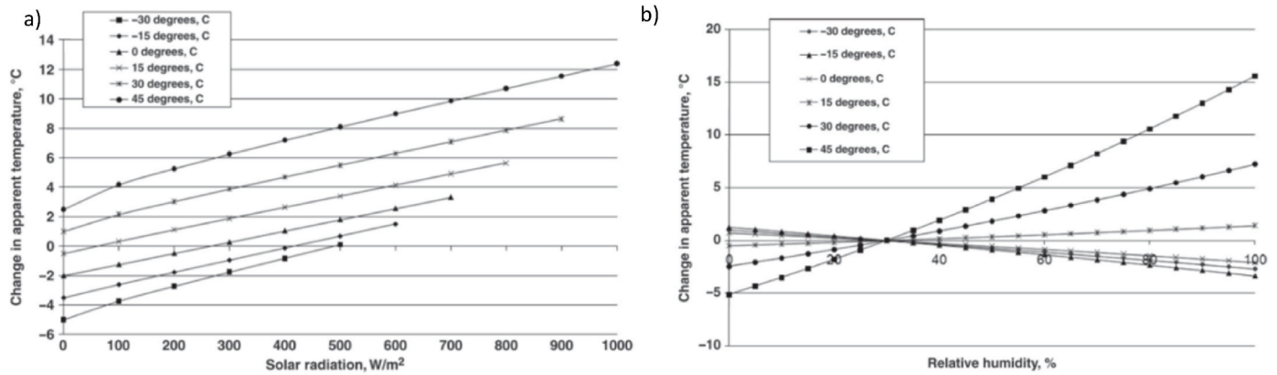
Fig. 1. Apparent temperature changes as (a) solar radiation and (b) relative humidity increases at varying ambient temperatures. Note. Sourced from A comprehensive index for assessing environmental stress in animals , by T. L. Mader, L. J. Johnson, and J. Gaughan, 2010, Journal of Animal Science , 88(6) pp 2155-2156.
