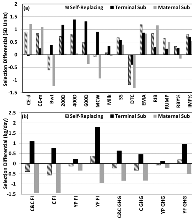
Figure 2. Selection differentials between top 10% and full published Hereford sire list ranked on the self-replacing index (base), the terminal sub-index (TSub) or the maternal sub-index (M-Sub) for (a) the BREEDPLAN EBVs and (b) estimated daily feed intake and greenhouse gas emissions. Traits: CE-d: calving ease-direct, CE-m: calving ease-maternal, Bwt: birth weight, 200D: 200-day weight, 400D: 400-day weight, 600D: 600-day weight, MCW: mature cow weight, Milk: 200-day maternal weight, SS: scrotal size, DTC: days-to-calving, EMA: eye muscle area, RIB: rib fat depth, RUMP: rump fat depth, RBY%: retail beef yield percentage, IMF%: intramuscular fat percentage, C&C: cow and calf at pasture, C: only cow at pasture, YP: young animal at pasture, YF: young animal in feedlot, FI: feed intake and GHG: GHG emissions.
