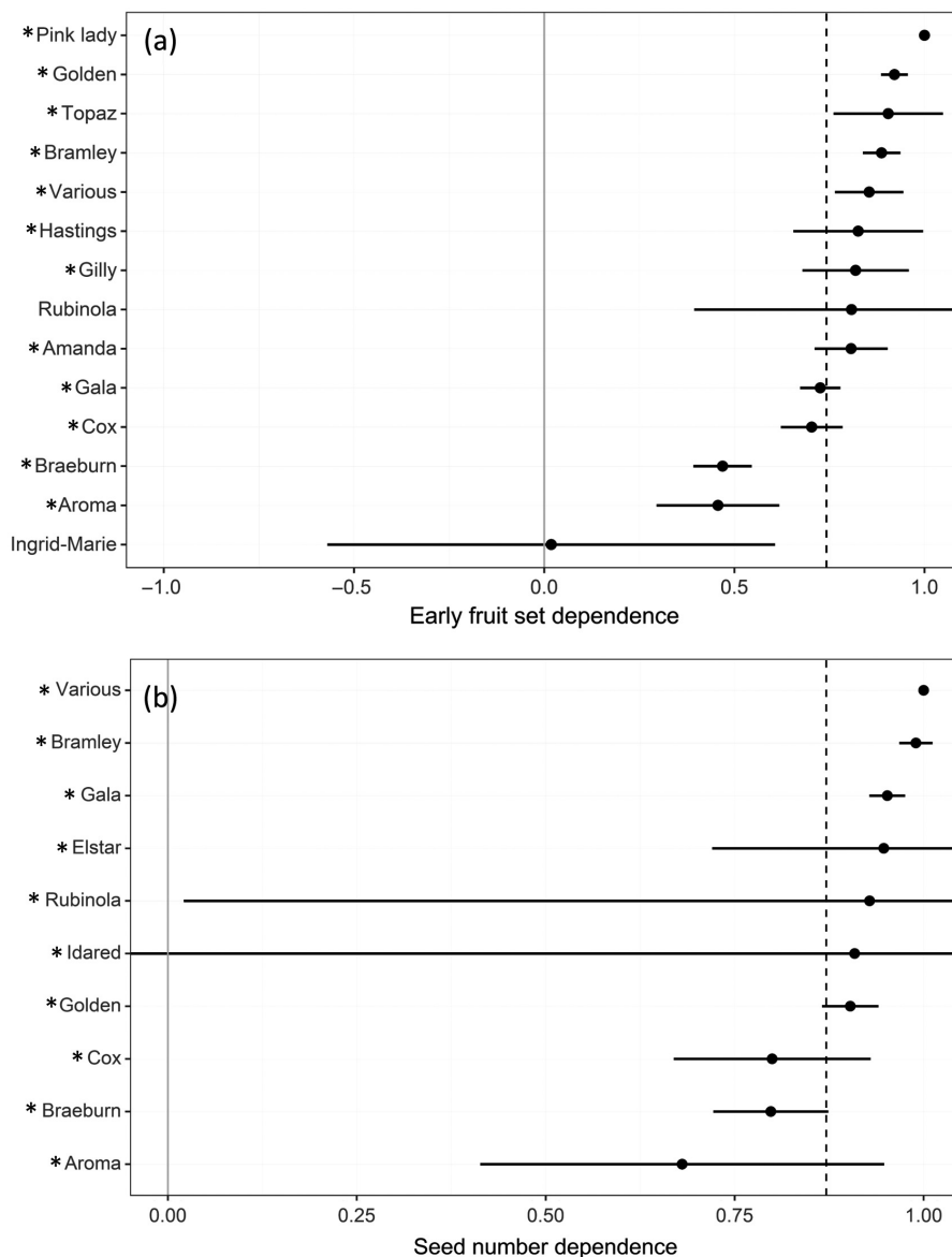
FIG. 4. The extent to which early fruit set (a) and seed number (b) of different apple varieties depend on pollination using available data from all orchards and countries. Mean pollinator dependence and 95% CI are shown for each variety and grand mean across varieties shown as a dashed line. Varieties marked with “*” indicate those with significant differences found between supplementary pollination and pollinator exclusion treatments ( P < 0.05 ).
