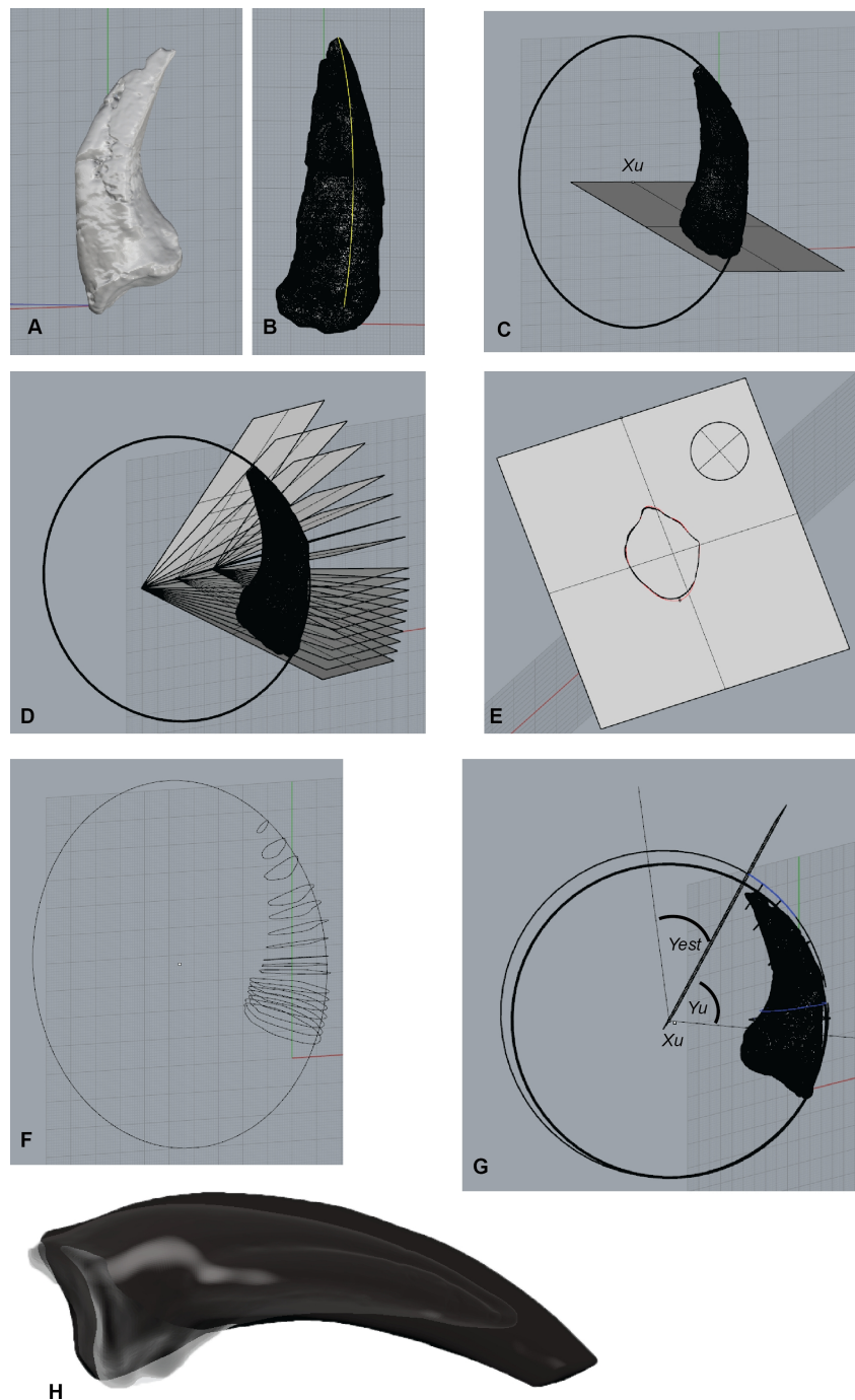
Figure 3 Australovenator unguis and sheath restoration. (A) Pedal unguis II-3 imported into Rhinoceros 5.0. (B) Outer surface curve drawn to dorsal unguis surface. (C) Circle attached to the best fit of outer curve of the unguis. (D) Section planes drawn from a centre point of the drawn circle. (E) Section through the unguis displaying the outer surface of the unguis. (F) Cross-section ribs of the unguis redrawn to represent unbroken sections. (G) A perfect circle was dorsally offset to the claw's rim for sheath thickness in Rhinoceros 5.0. The offset synthesized the dorsal sheath thickness which was progressive until the sheath's tip. (H) Wear facets on the reconstructed sheaths. Abbreviations: Centre of circle ( Xu ), Ungual angle ( Yu ), Sheath extent ( Yest ).
