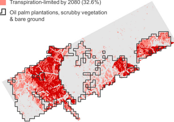
(c) RCP8.5 scenario (+2.8°C by 2080) assuming 12 hPa threshold to transpiration
