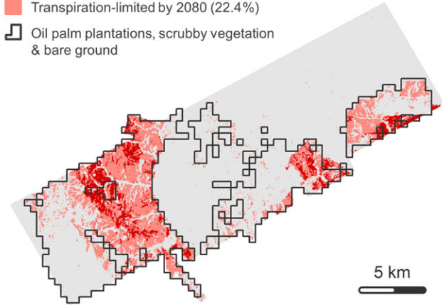
FIGURE 5 Areas of the SAFE landscape where mean maximum daily vapour pressure deficit ( VPD_{max} ) is predicted to exceed hypothesized transpiration thresholds (12 and 15 hPa) for tree seedlings under current (dark red) and future climate conditions (light red). Results for two different IPCC representative concentration pathways (RCP) are shown: the RCP4.5 emission mitigation scenario (a and b) and the RCP8.5 business-as-usual scenario (c and d). The percentage of 50 \times 50 m pixels exceeding VPD_{max} thresholds is given in brackets for each scenario. The black contour lines mark the current extent of oil-palm plantations within the SAFE landscape, as well as areas dominated by short scrubby vegetation that develops in the aftermath of logging and of bare ground [Colour figure can be viewed at wileyonlinelibrary.com ]
