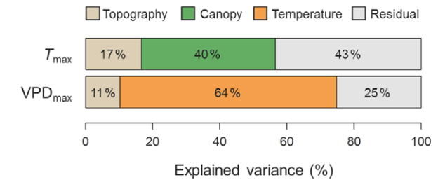
FIGURE 1 Piecewise structural equation models relating variation in (a) annual mean temperature ( T_{\text{mean}} ) and vapour pressure deficit ( \text{VPD}_{\text{mean}} ) and (b) mean maximum daily temperature ( T_{\text{max}} ) and vapour pressure deficit ( \text{VPD}_{\text{max}} ) to canopy structural and topographic metrics. The models also capture the effects of logging pressure and land-use intensity on maximum canopy height ( H_{\text{max}} ), as well as the covariation between H_{\text{max}} and plant area index (PAI)—which was explicitly accounted for by taking the residuals of a regression relating PAI to H_{\text{max}} as a predictor of temperature and VPD in the models. Dark grey arrows denote positive relationships, while light ones correspond to negative associations. The width of the arrows reflects the strength of the pathway and is proportional to the standardized path coefficient (reported in Appendix S3). A dashed arrow was used to represent the interaction effect between aspect and H_{\text{max}} . Only pathways that were significant to p \leq 0.05 are shown. R^2 values are reported for each endogenous variable. Additionally, panels (b) and (d) provide a breakdown of how much of the variance in T_{\text{mean}} , \text{VPD}_{\text{mean}} , T_{\text{max}} and \text{VPD}_{\text{max}} was explained by topographic metrics, canopy structural metrics and (in the case of VPD) by temperature [Colour figure can be viewed at wileyonlinelibrary.com ]
