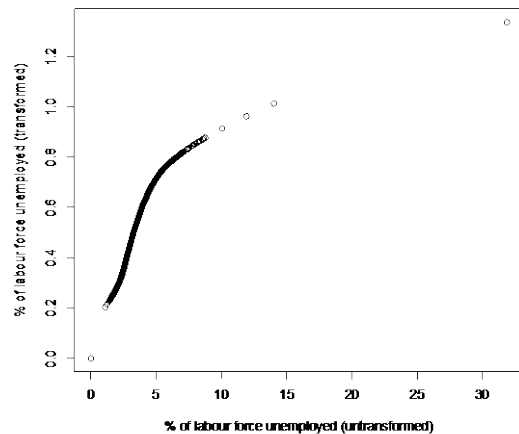
Scatter plot of transformed and untransformed indicator values
