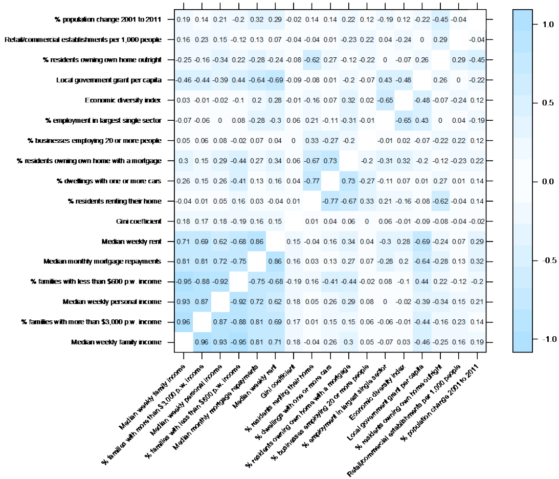
Figure 3.5: Example correlation level plot for the economic capital theme indicators.
