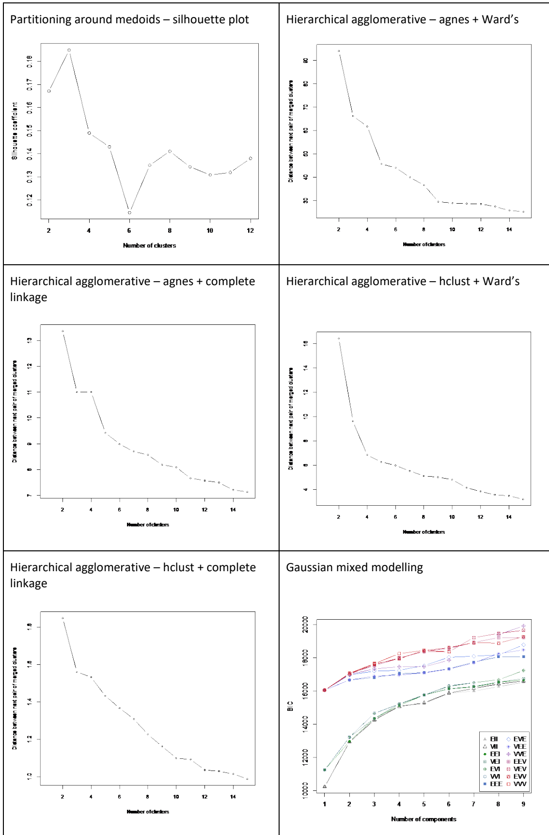
Figure 3.11: Comparison of cluster outcomes from different clustering methods.
