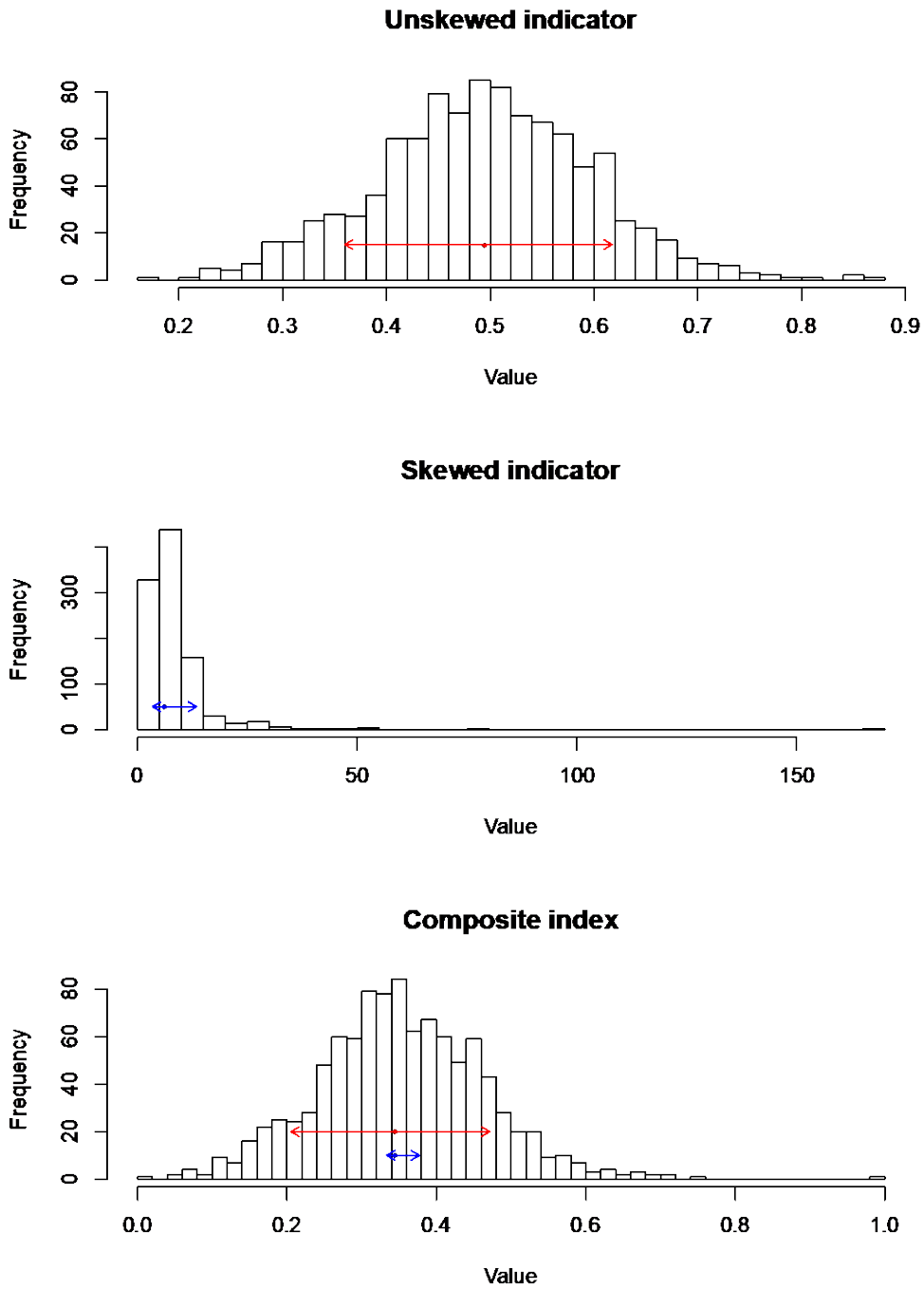
Figure 3.1: Histograms of an unskewed indicator, a skewed indicator and the resulting composite index. For the unskewed indicator, the red dot and arrows show the positions of the median and first and ninth decile values. For the skewed indicator, the positions of the same quantiles are shown similarly in blue. For the composite index, the dots and arrows show the changes in the index as each indicator in turn is changed from its median value to its first decile or ninth decile value.
