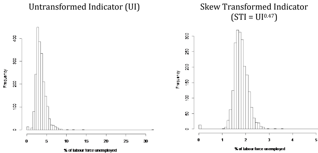
Figure 3.3: Histograms of the ‘% of labour force unemployed’ indicator before and after transformation.
