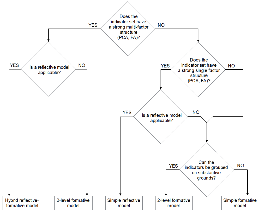
Figure 3.6: Decision tree for choice of measurement model.
