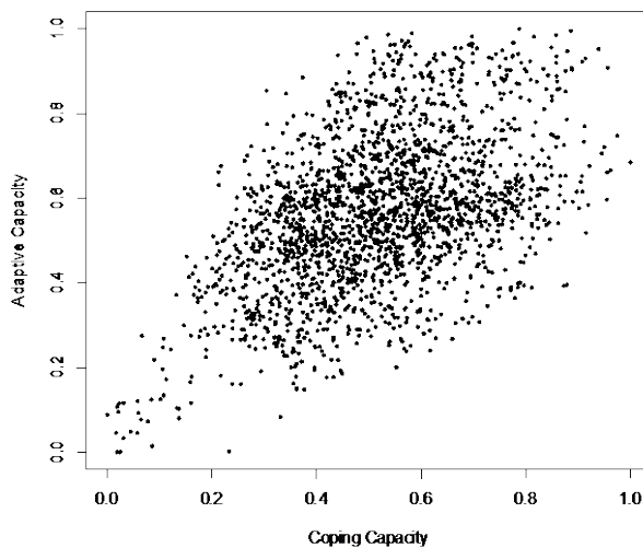
Figure 3.9: Scatterplot of coping and adaptive capacity index values demonstrating lack of cluster structure.
