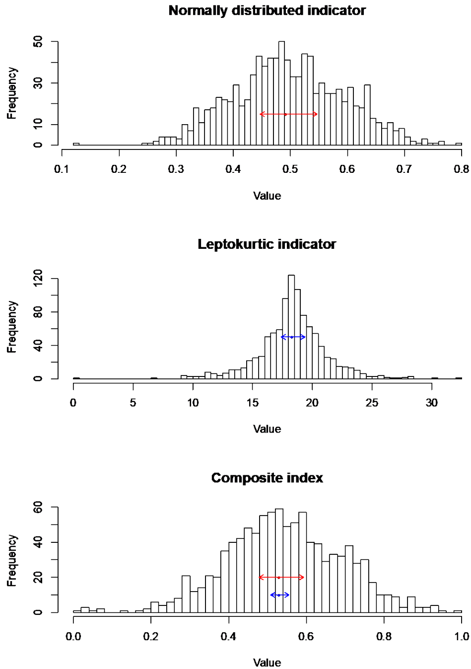
Figure 3.2: Histograms of a normally distributed indicator, a leptokurtic indicator and the resulting composite index. For the normally distributed indicator, the red dot and arrows show the positions of the median and third and seventh decile values. For the leptokurtic indicator, the positions of the same quantiles are shown similarly in blue. For the composite index, the dots and arrows show the changes in the index as each indicator in turn is changed from its median value to its third decile or seventh decile value.
