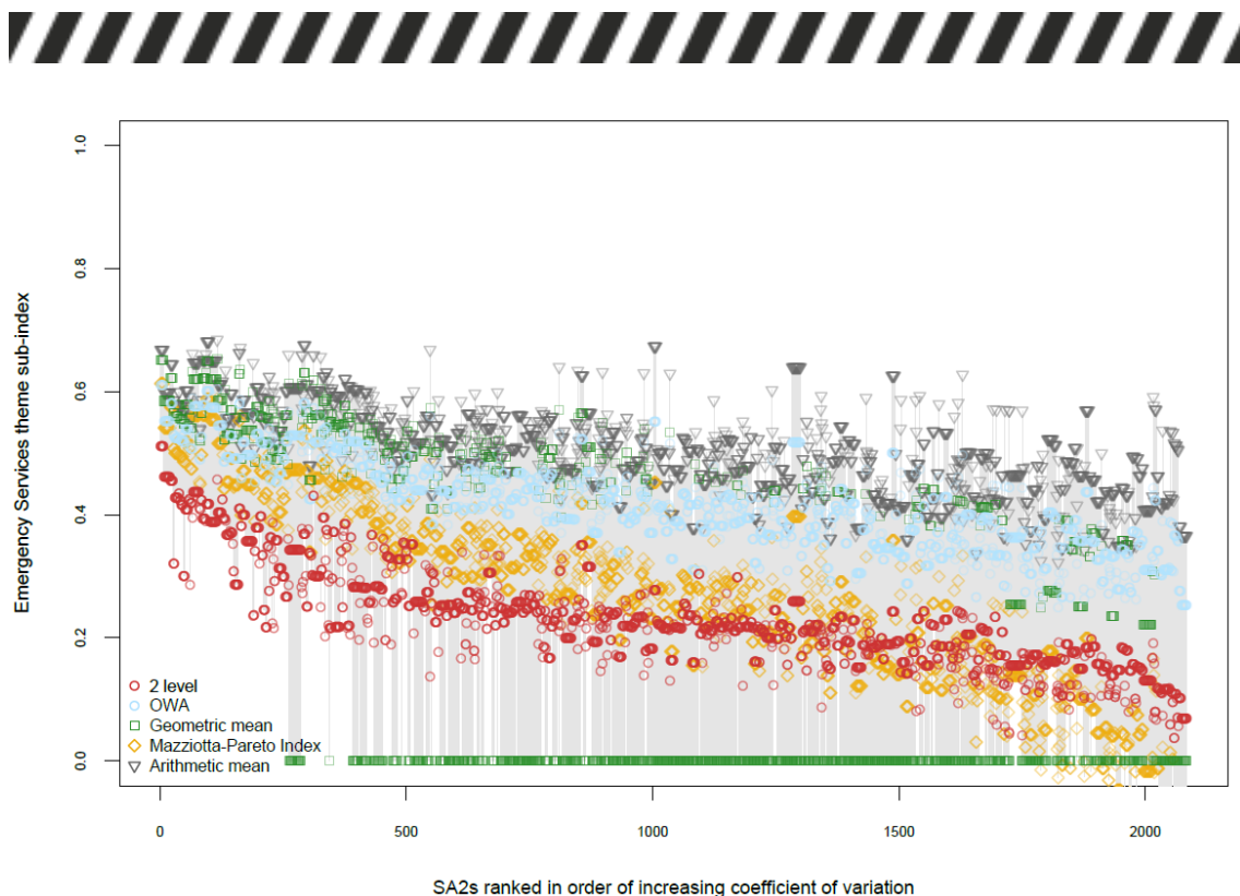
Figure 3.8: Example of comparison of the chosen aggregation method (a two level formative model with aggregation by OWA and discrete Choquet integral (denoted as 2 level in the key) with alternative methods of aggregation. SA2s are ordered according to the coefficient of variation of their indicators, lowest to the left and highest to the right.
