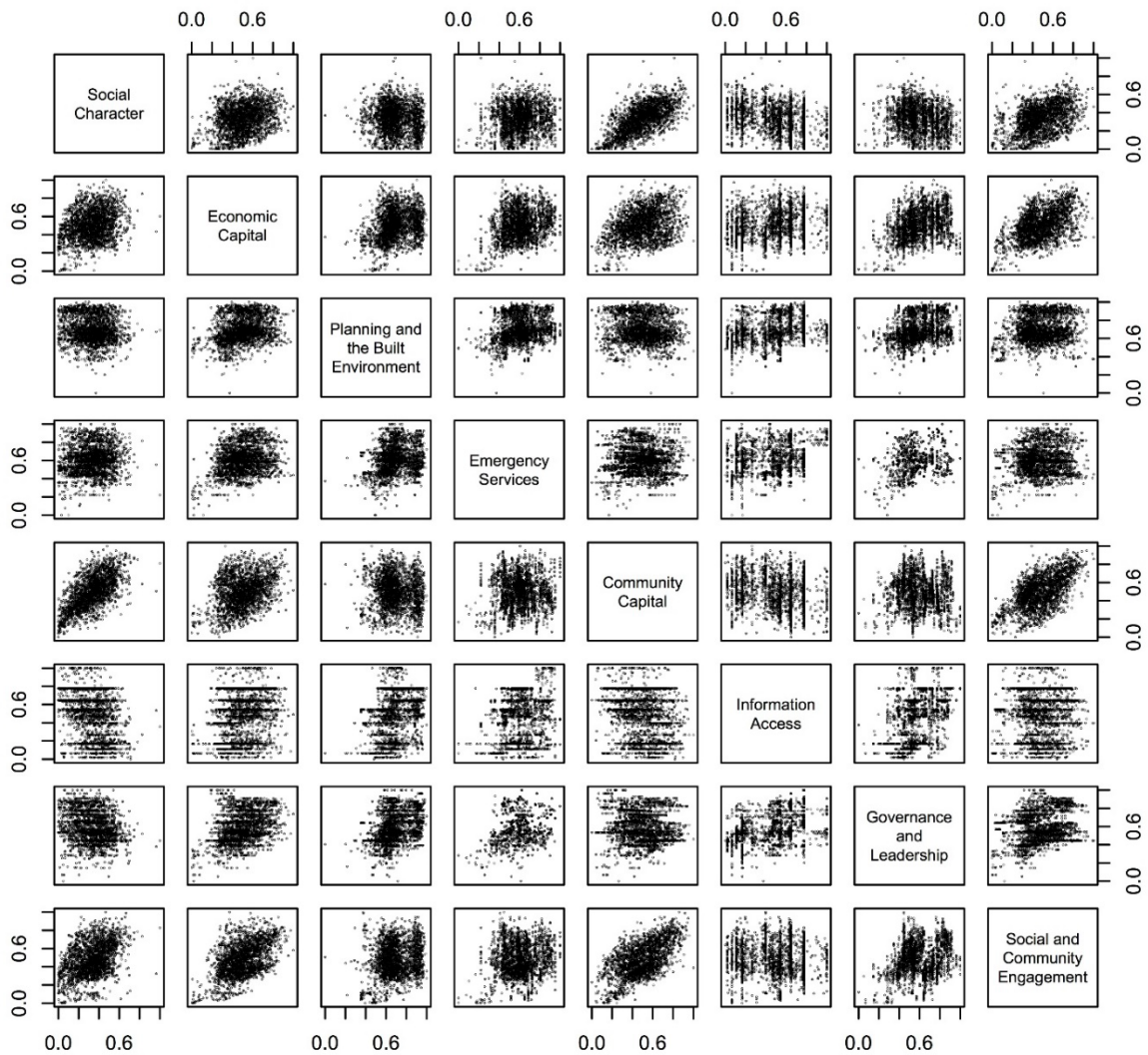
Figure 3.10: Theme level paired scatterplots showing potential cluster structure.
