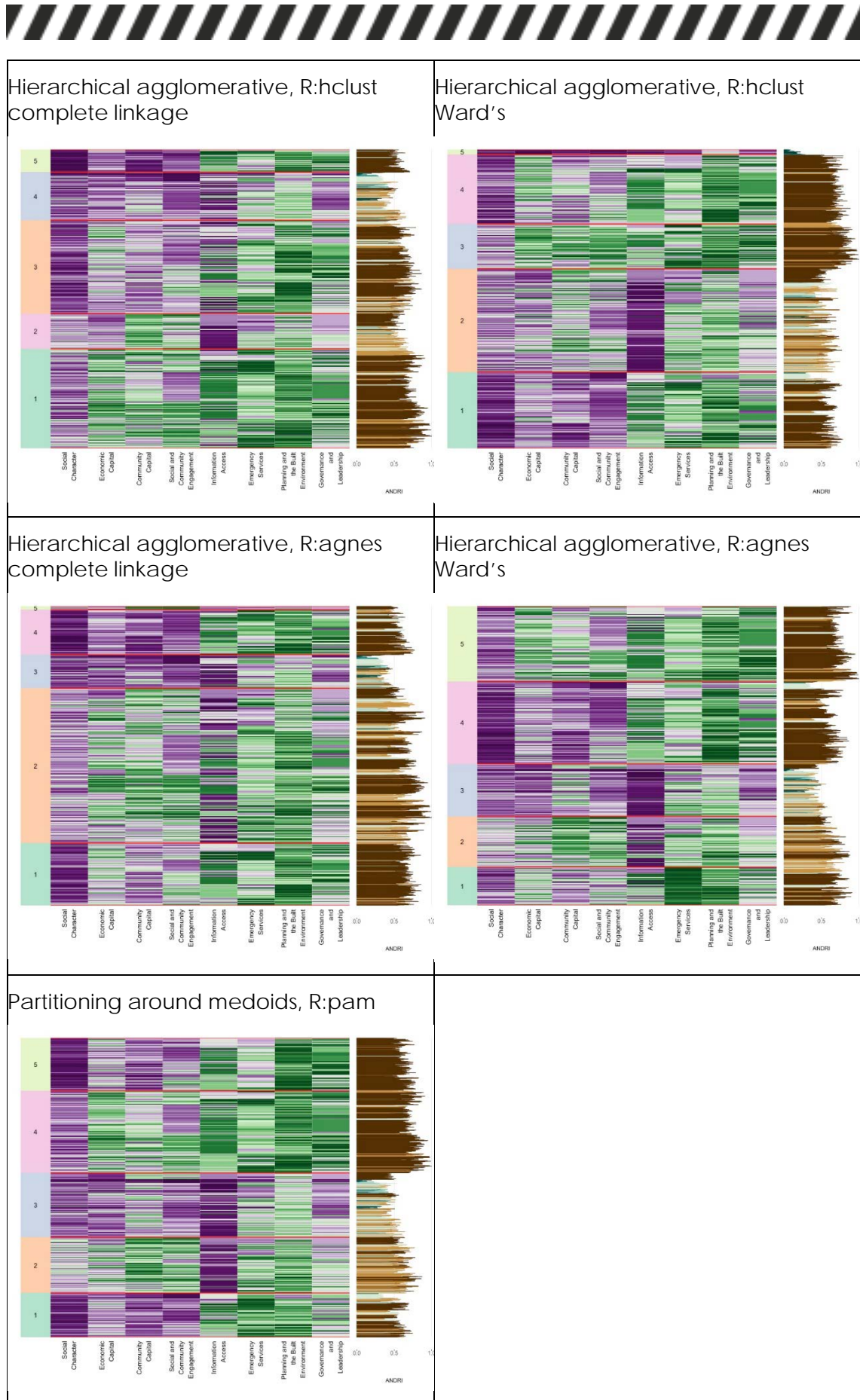
Figure 3.12: Caption on following page
