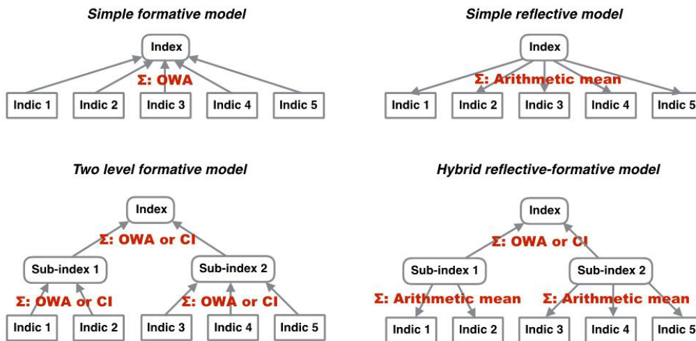
Figure 3.7: Aggregation strategies considered and/or tested in the computation of the Australian Natural Disaster Resilience Index. Arrows denote the direction of causation implicit in the model. Options for the aggregation method within each model are shown in red. OWA = Ordered Weighted Average, CI = Choquet Integral.
