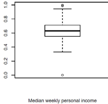
Transformed distribution
