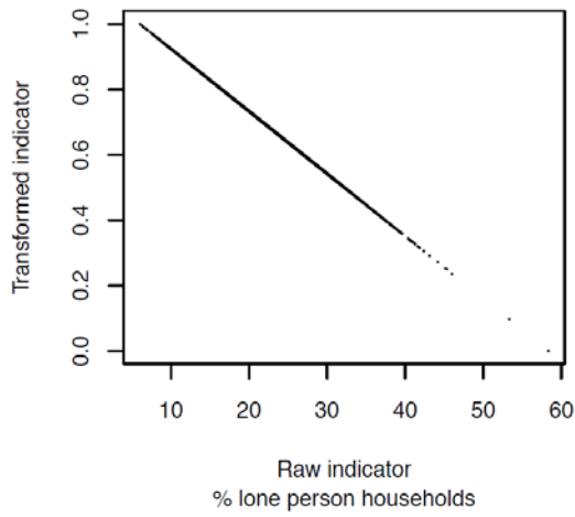
Transformation relationship
