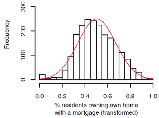
Transformed distribution
