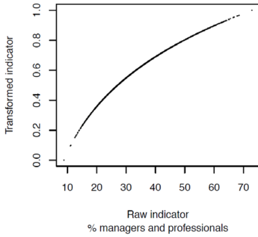
Transformation relationship
