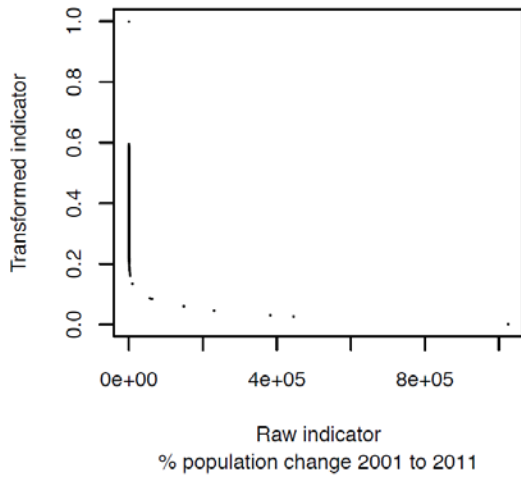
Transformation relationship
