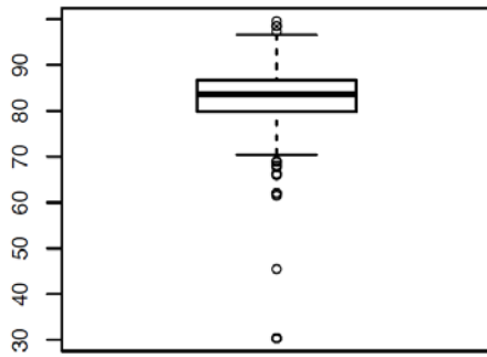
Raw distribution
