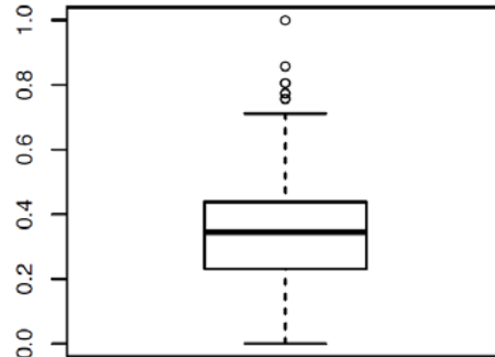
Transformed distribution
