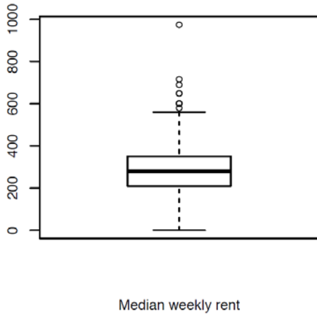
Raw distribution
