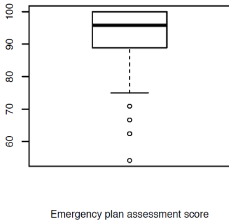
Raw distribution
