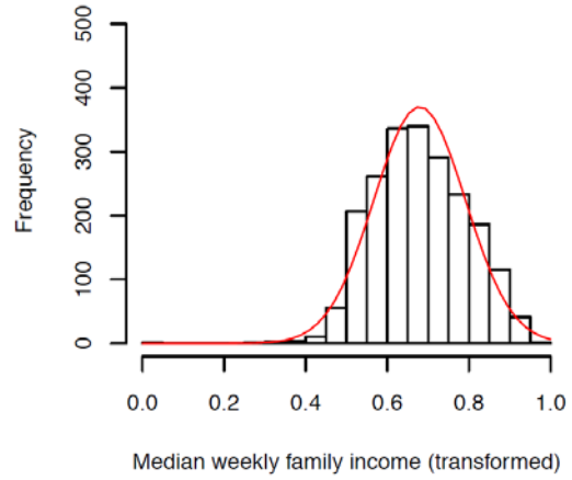
Transformed distribution
