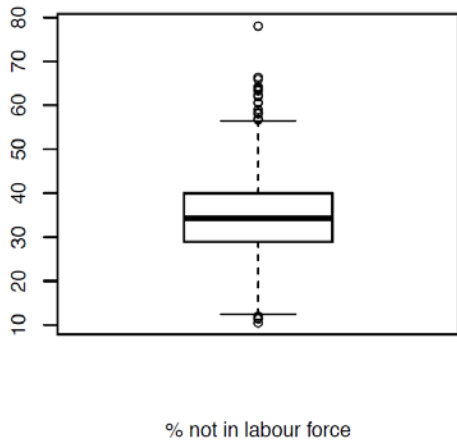
Raw distribution
