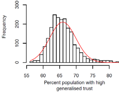
Raw distribution
