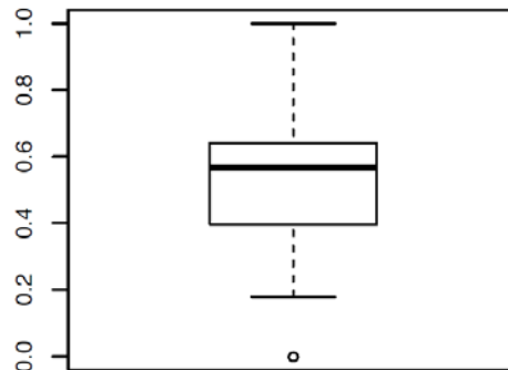
Transformed distribution
