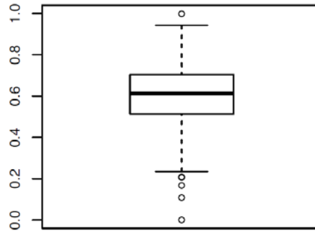
Transformed distribution
