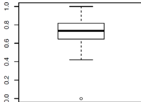
Transformed distribution
