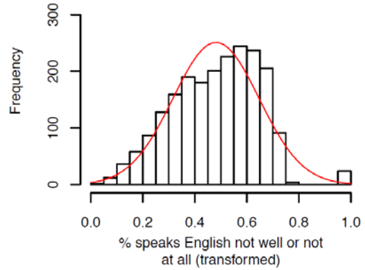
Transformed distribution
