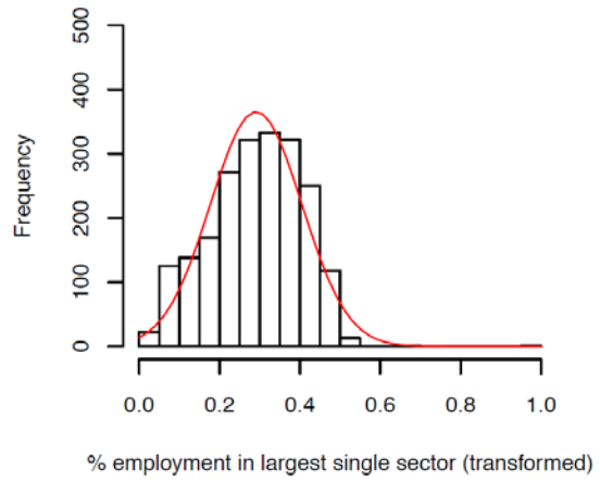
Transformed distribution
