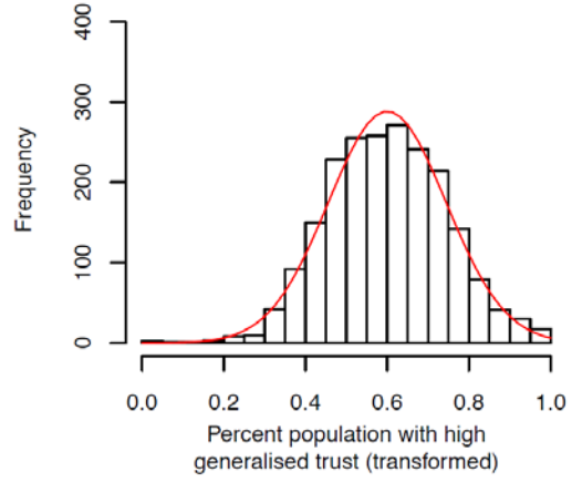
Transformed distribution
