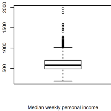
Raw distribution
