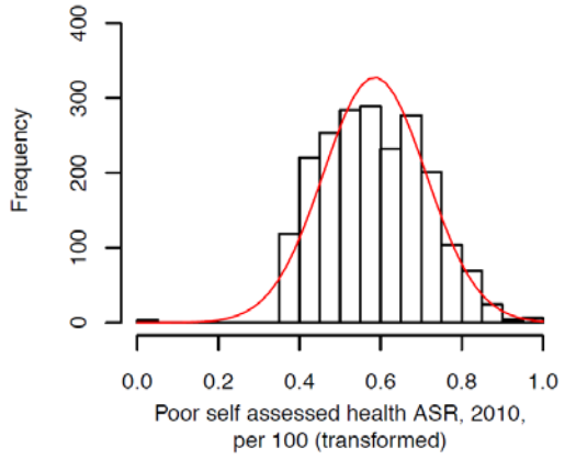
Transformed distribution
