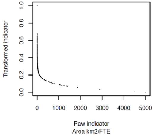
Transformation relationship
