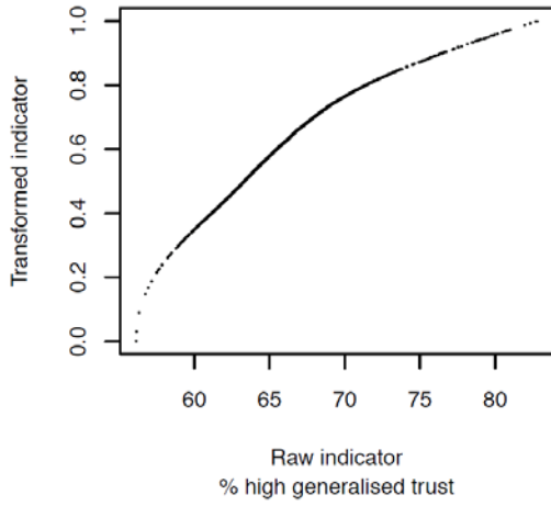
Transformation relationship
