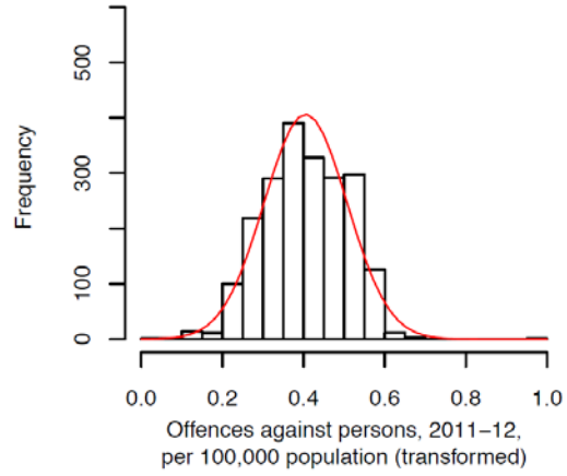
Transformed distribution
