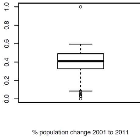
Transformed distribution
