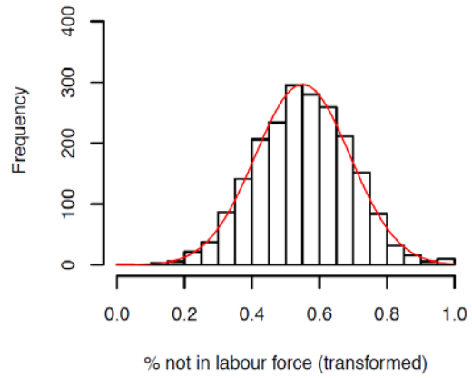
Transformed distribution
