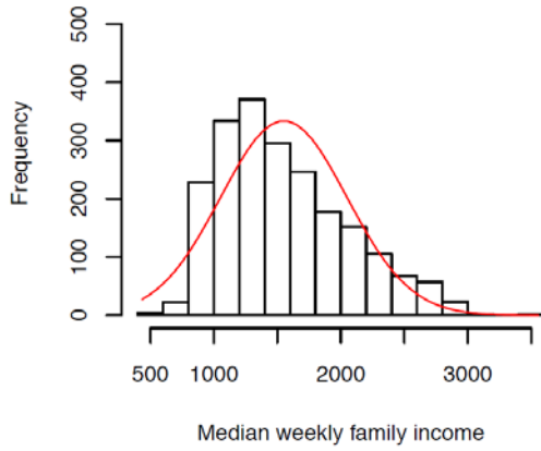
Raw distribution
