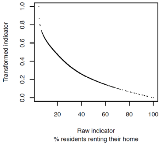
Transformation relationship
