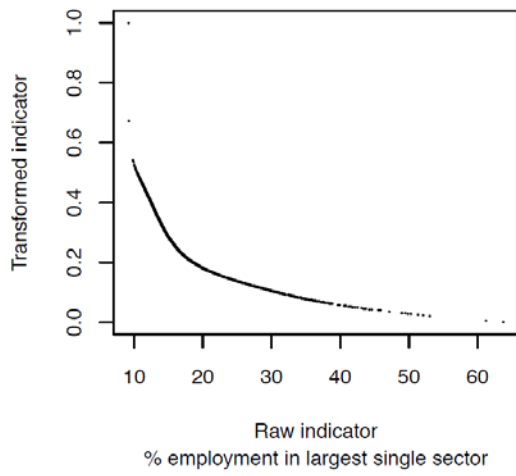
Transformation relationship
