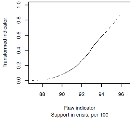
Transformation relationship
