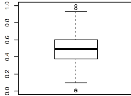
Transformed distribution
