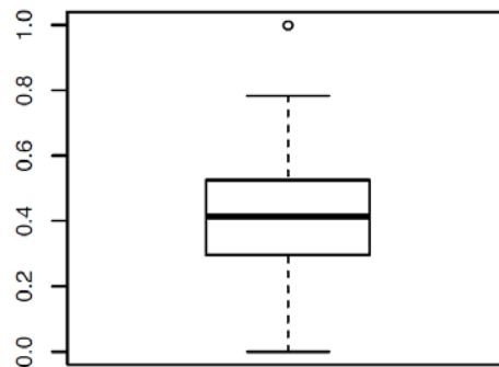
Transformed distribution
