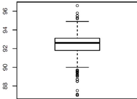
Raw distribution
