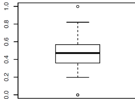
Transformed distribution
