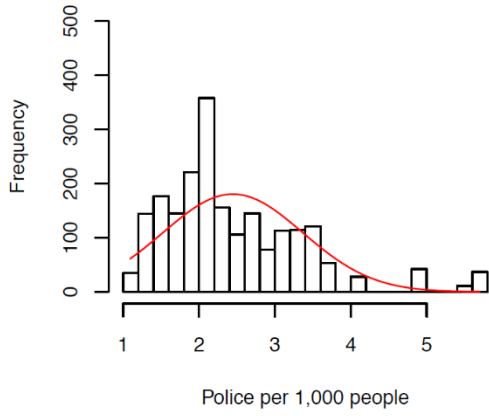
Raw distribution
