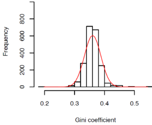
Raw distribution
