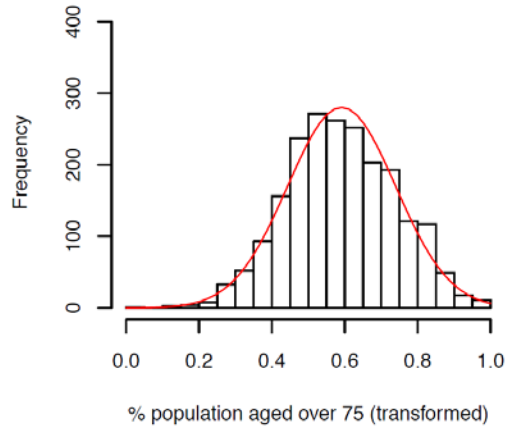
Transformed distribution
