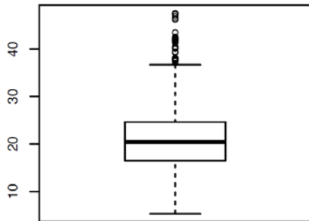
Raw distribution
