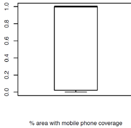
Transformed distribution
