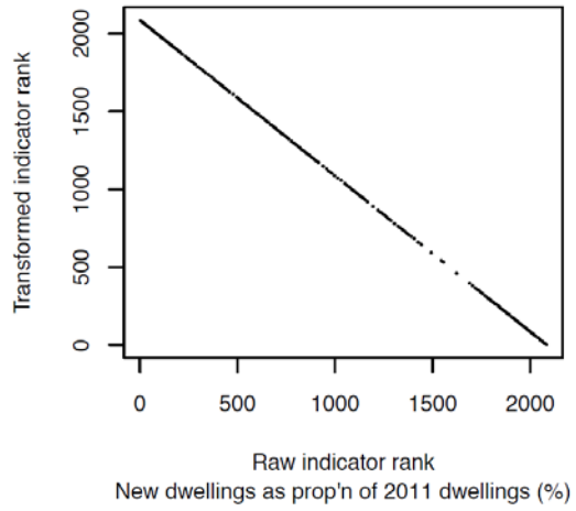
Order preservation check
