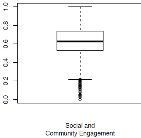
Raw distribution
