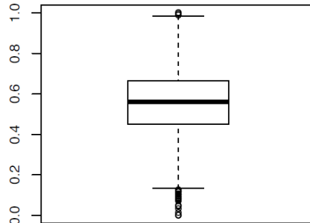
Transformed distribution
