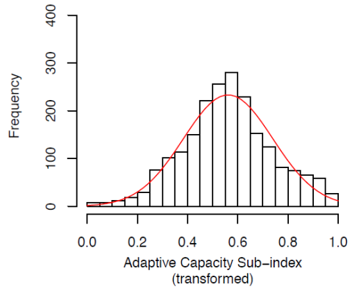
Transformed distribution
