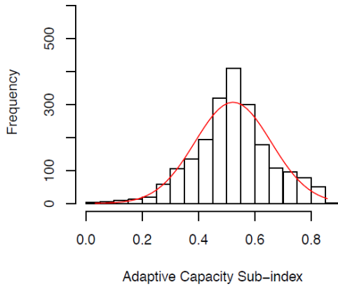
Raw distribution
