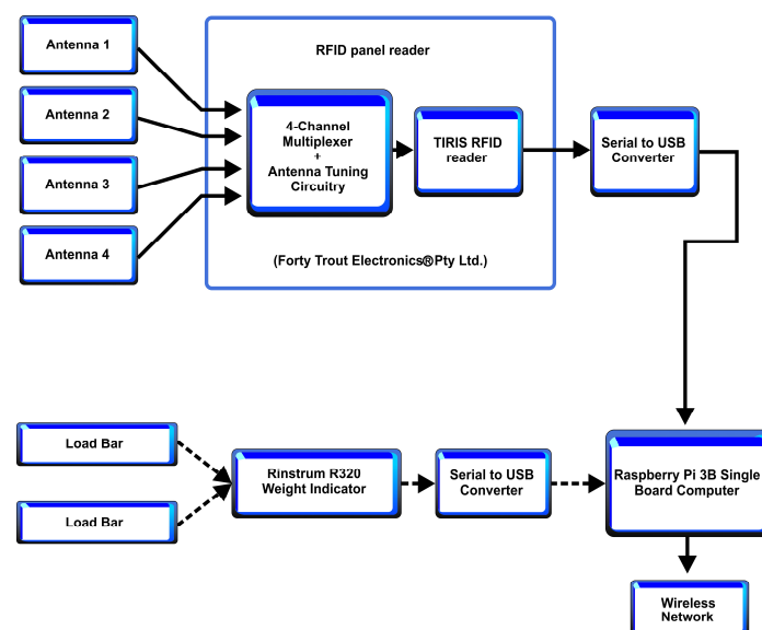
Figure 3. Schematic of the automatic supplement weighing (ASW) unit hardware.
