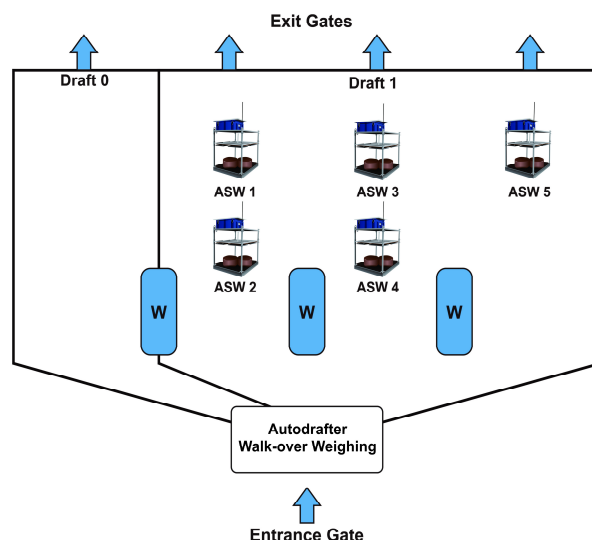
Figure 4. The layout of the experimental sites where the automatic supplement weighing (ASW) units, water troughs (W), and walk-over weighing were installed on each site. The total area of Draft 0 and Draft 1 was 3500 and 10,500 m 2 , respectively.
