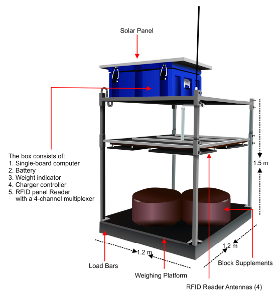
Figure 2. The layout of the automatic supplement weighing (ASW) unit.
