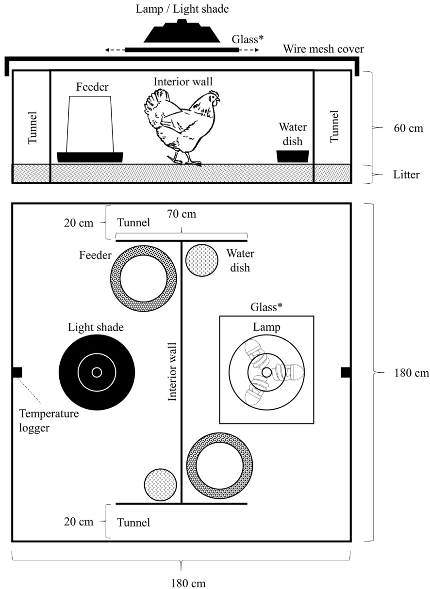
Figure 1. A schematic of the Light Preference Testing Apparatus (LPTA) showing the dimensions of the LPTA and placement of the food, water, lights and temperature loggers. *For the UVA treatments, 3-mm glass was placed between the lamp and the wire mesh cover to filter the UVB wavelengths.
