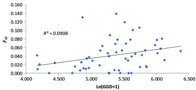
FIGURE 3 Mantel tests showing the relationship between pairwise genetic distance and natural log-transformed geographic distance in 11 subpopulations of lignum ( Duma florulenta ) in the northern Murray–Darling Basin
