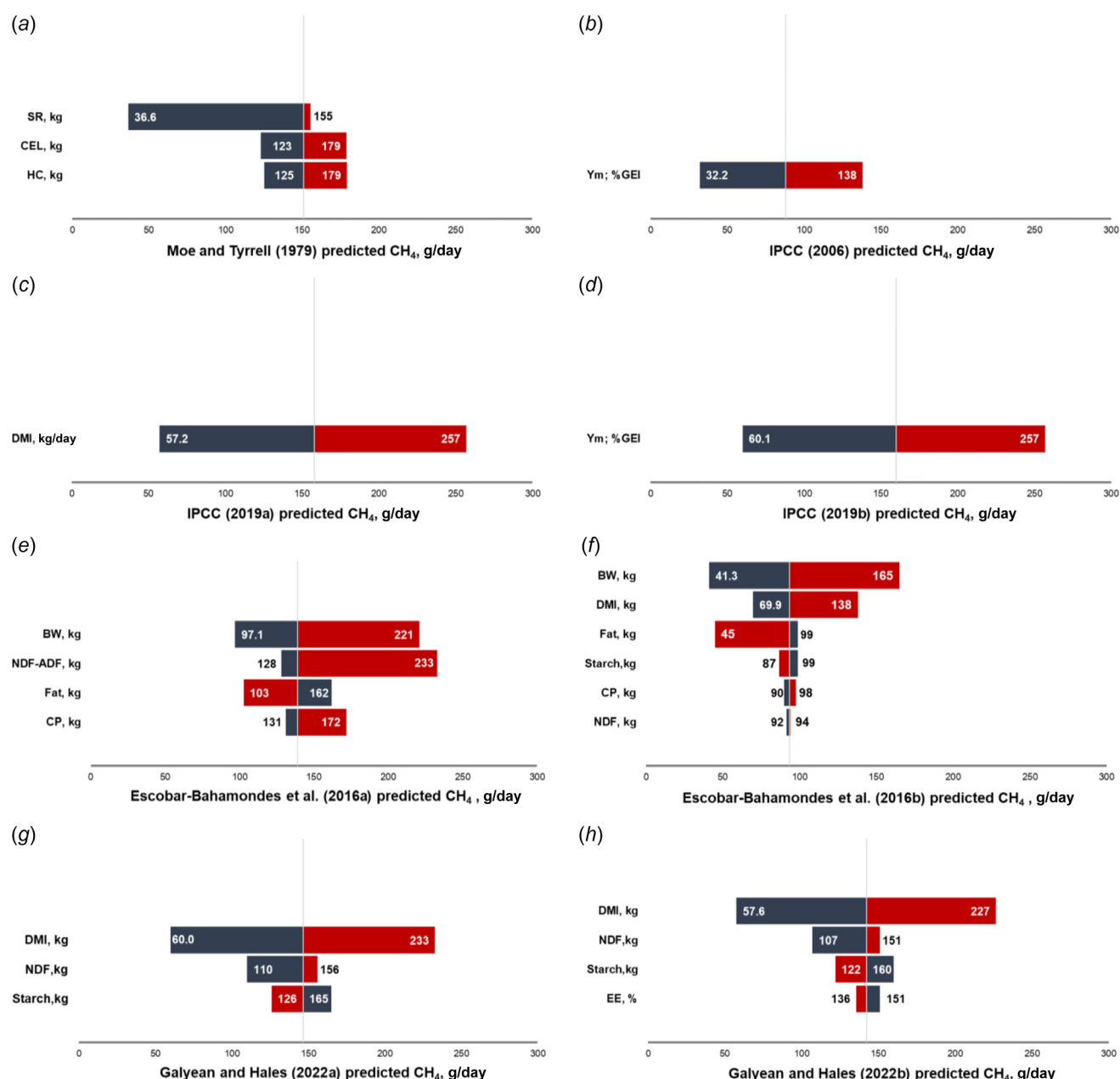
Fig. 3. Tornado plot depicting low (blue zone) and high (red zone) input variables of existing equations to predict daily CH 4 emission (g) in feedlot cattle. White values inside the blue and red bars represent the predicted CH 4 emission (g/day) at the minimum (blue) and maximum (red) values of each input variable. GEI = gross energy intake, SR = soluble residue, CEL = cellulose, HC = hemicellulose, DMI = dry matter intake, BW = body weight, NDF = neutral detergent fibre, ADF = acid detergent fibre, CP = crude protein, STA = starch.
