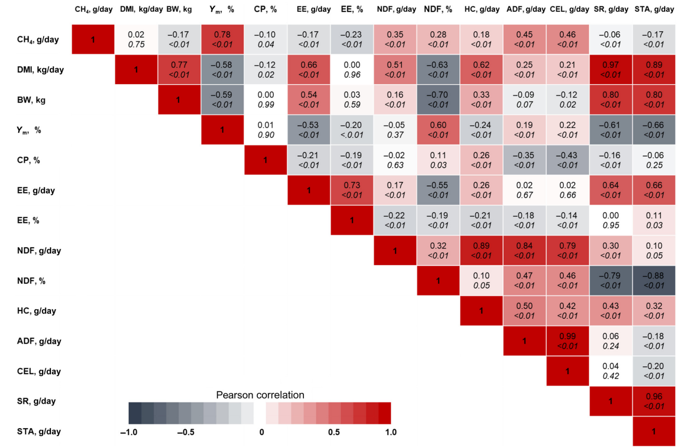
Fig. 2. Linear relationship (Pearson correlation = r ) of input variables required to predict methane in evaluated literature equations. CH 4 = methane, DMI = dry matter intake, BW = body weight, Y m = emission factor, CP = crude protein, EE = ether extract, NDF = neutral detergent fibre, HC = hemicellulose, ADF = acid detergent fibre, CEL = cellulose, SR = soluble residue, STA = starch.
