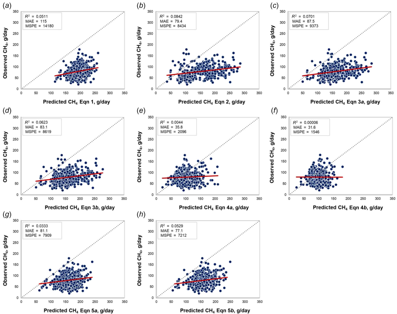
Fig. 1. Plot of observed CH 4 (g/day) vs predicted CH 4 (g/day) from literature equations. r^2 = coefficient of determination, MAE = mean absolute error, MSPE = mean square prediction error.
