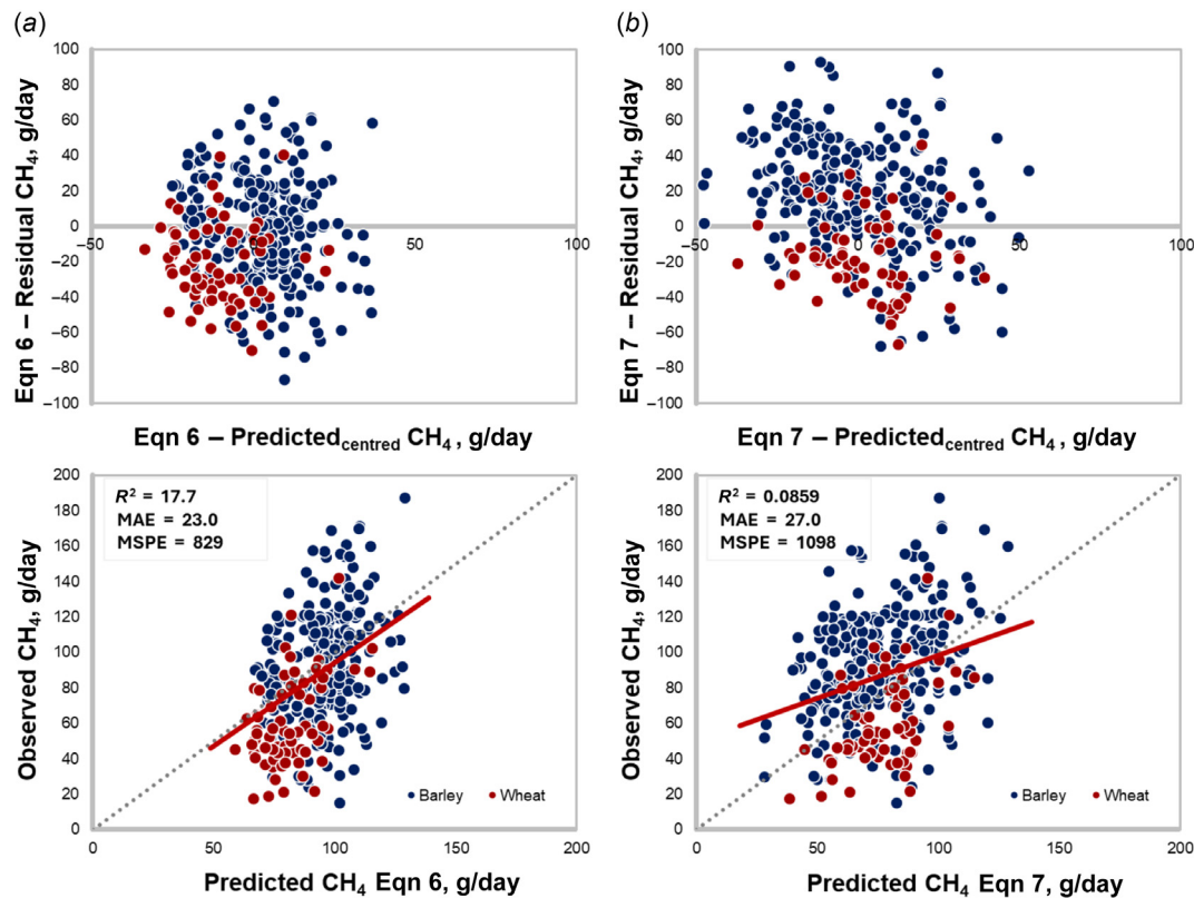
Fig. 5. Validation of Eqs 6 (a), 7 (b) using the independent dataset. MAE = mean absolute error, MSPE = mean square prediction error.
