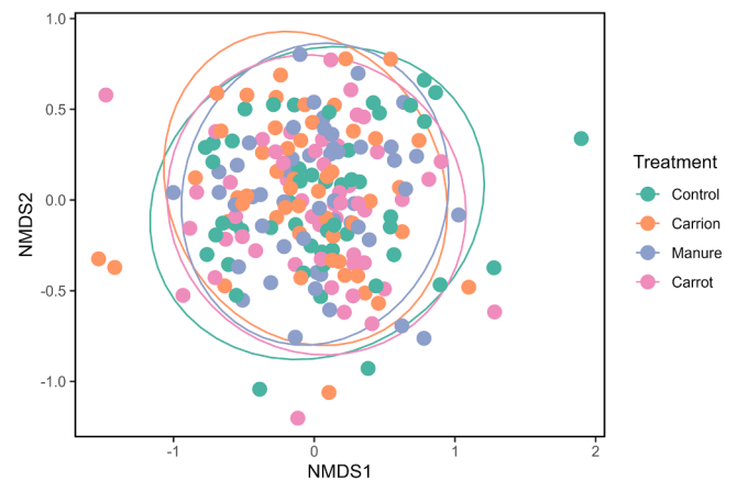
Fig. 2. NMDS plot comparing insect community composition on carrot umbels around the treatments (control (no resource), carrion, manure, and carrot material).
