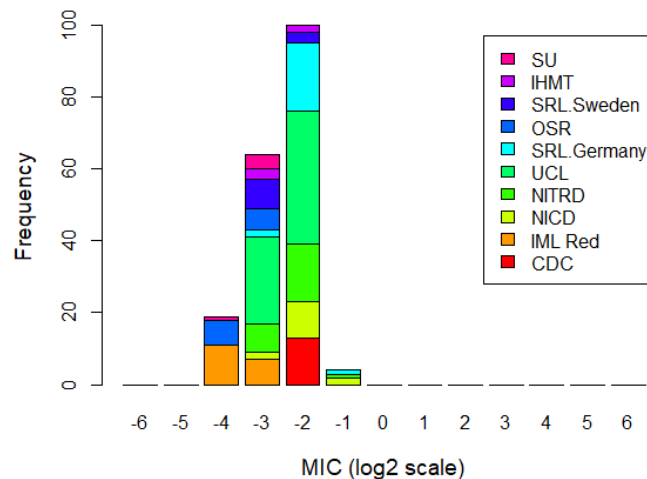
Figure 3. Aggregated MGIT MIC distribution of H37Rv
